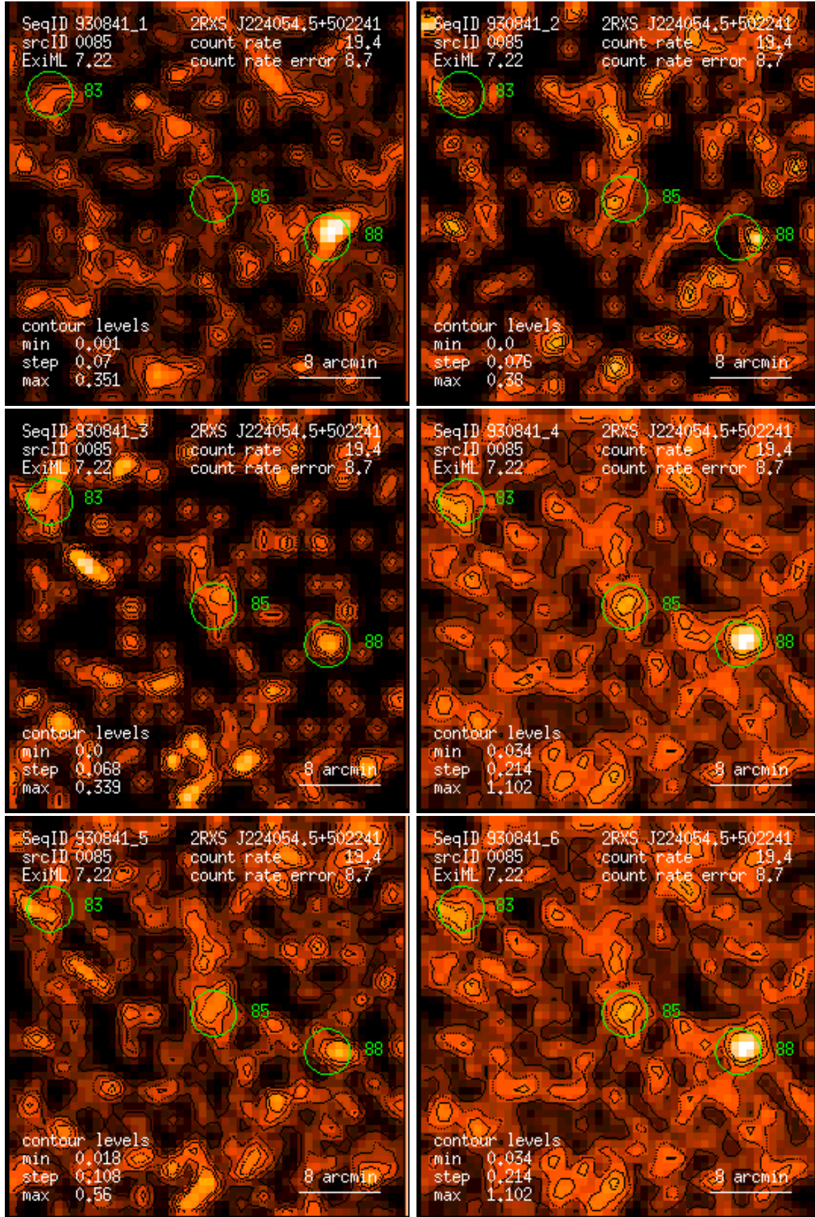
Figure 85: RASS 930841: detection 0085: band rate images, Gaussian filter: (1) PSPC channels 11 – 41, (2) 52 – 90, (3) 91 – 201, (4) 11 – 235, (5) 52 – 201, (6) 11 – 201. Broad band rates in counts/ks. Band rate contour levels in counts/ks/arcmin 2 .
