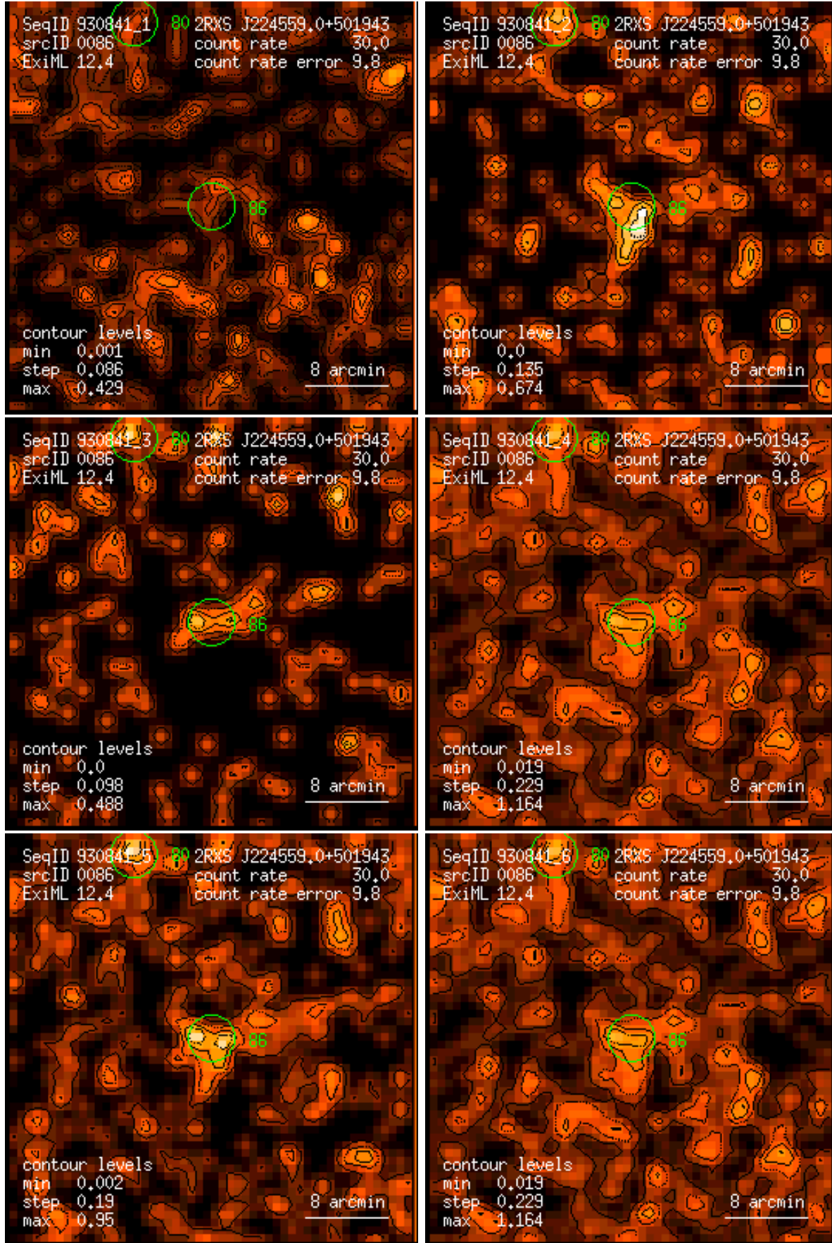
Figure 86: RASS 930841: detection 0086: band rate images, Gaussian filter: (1) PSPC channels 11 – 41, (2) 52 – 90, (3) 91 – 201, (4) 11 – 235, (5) 52 – 201, (6) 11 – 201. Broad band rates in counts/ks. Band rate contour levels in counts/ks/arcmin 2 .
