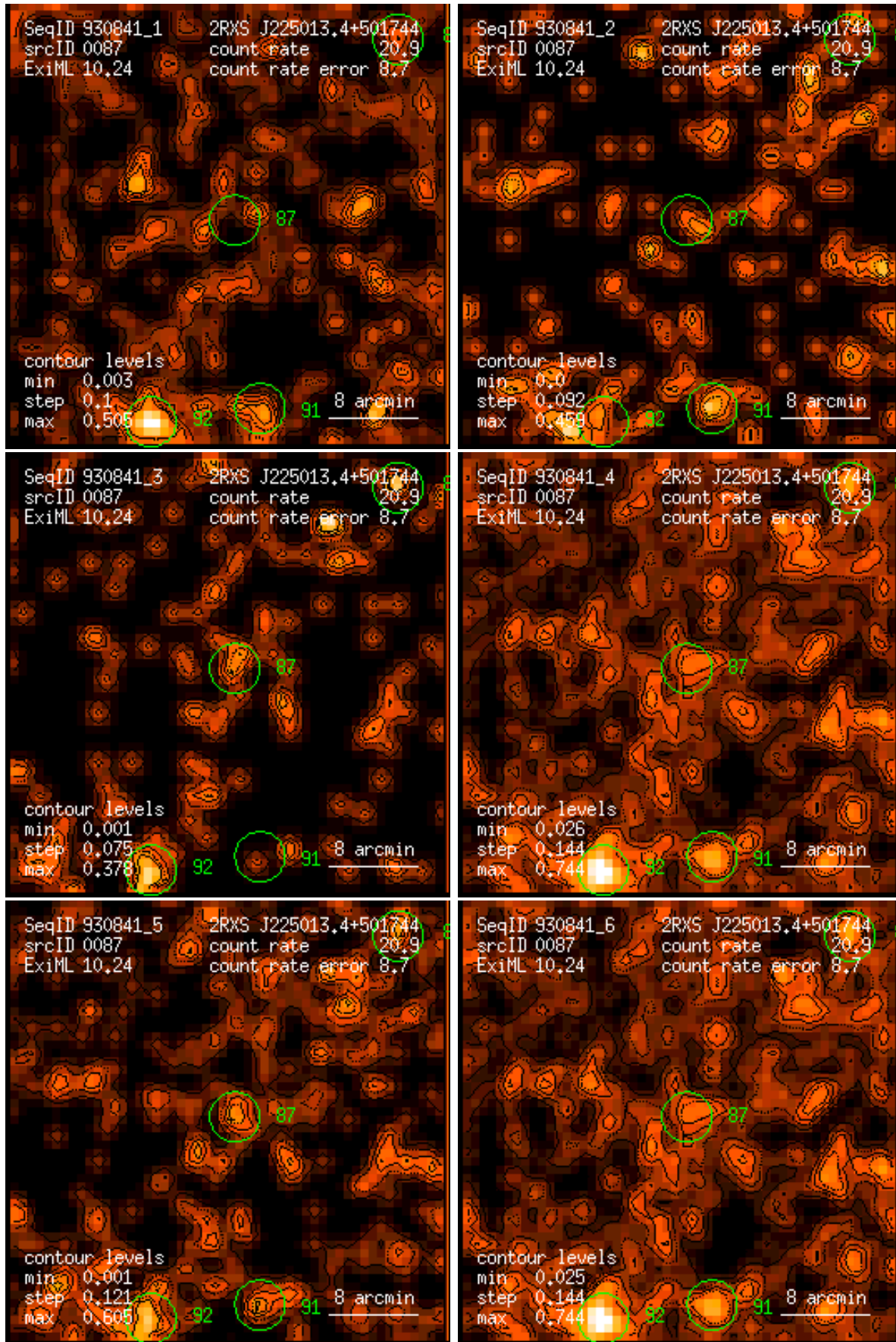
Figure 87: RASS 930841: detection 0087: band rate images, Gaussian filter: (1) PSPC channels 11 – 41, (2) 52 – 90, (3) 91 – 201, (4) 11 – 235, (5) 52 – 201, (6) 11 – 201. Broad band rates in counts/ks. Band rate contour levels in counts/ks/arcmin 2 .
