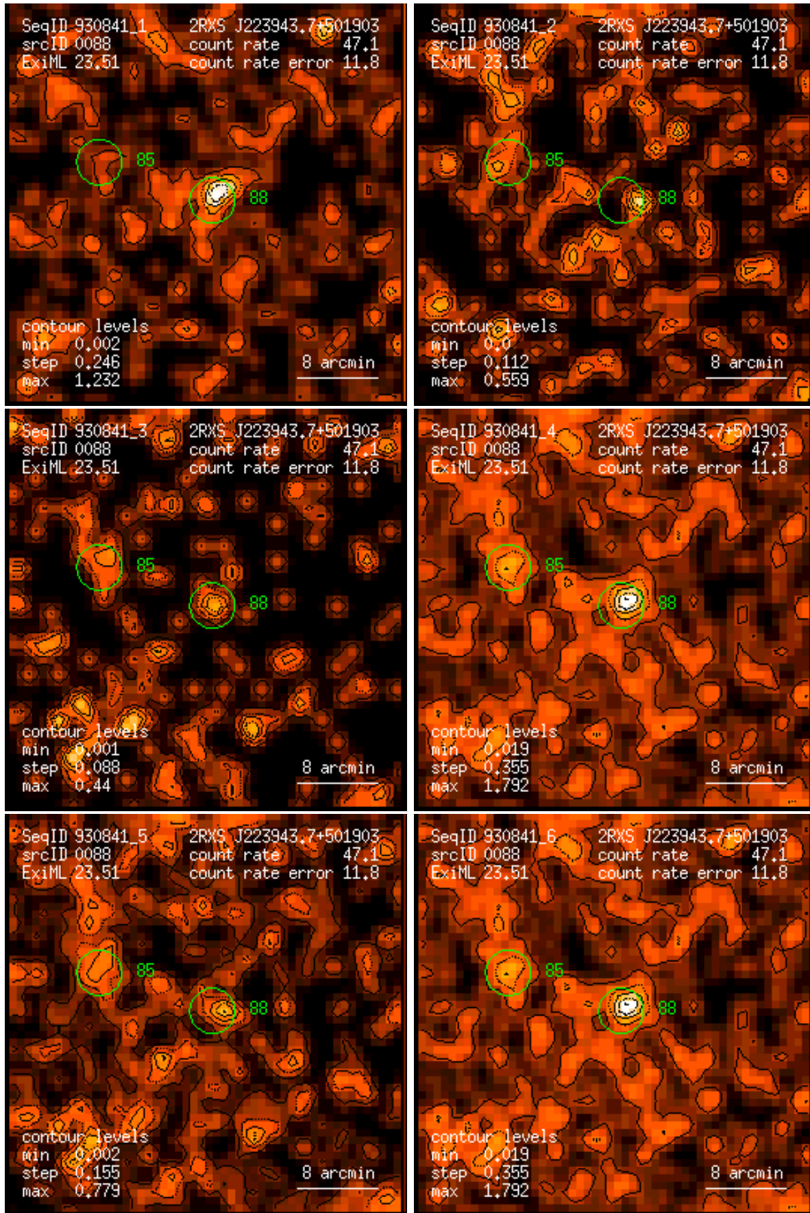
Figure 88: RASS 930841: detection 0088: band rate images, Gaussian filter: (1) PSPC channels 11 – 41, (2) 52 – 90, (3) 91 – 201, (4) 11 – 235, (5) 52 – 201, (6) 11 – 201. Broad band rates in counts/ks. Band rate contour levels in counts/ks/arcmin 2 .
