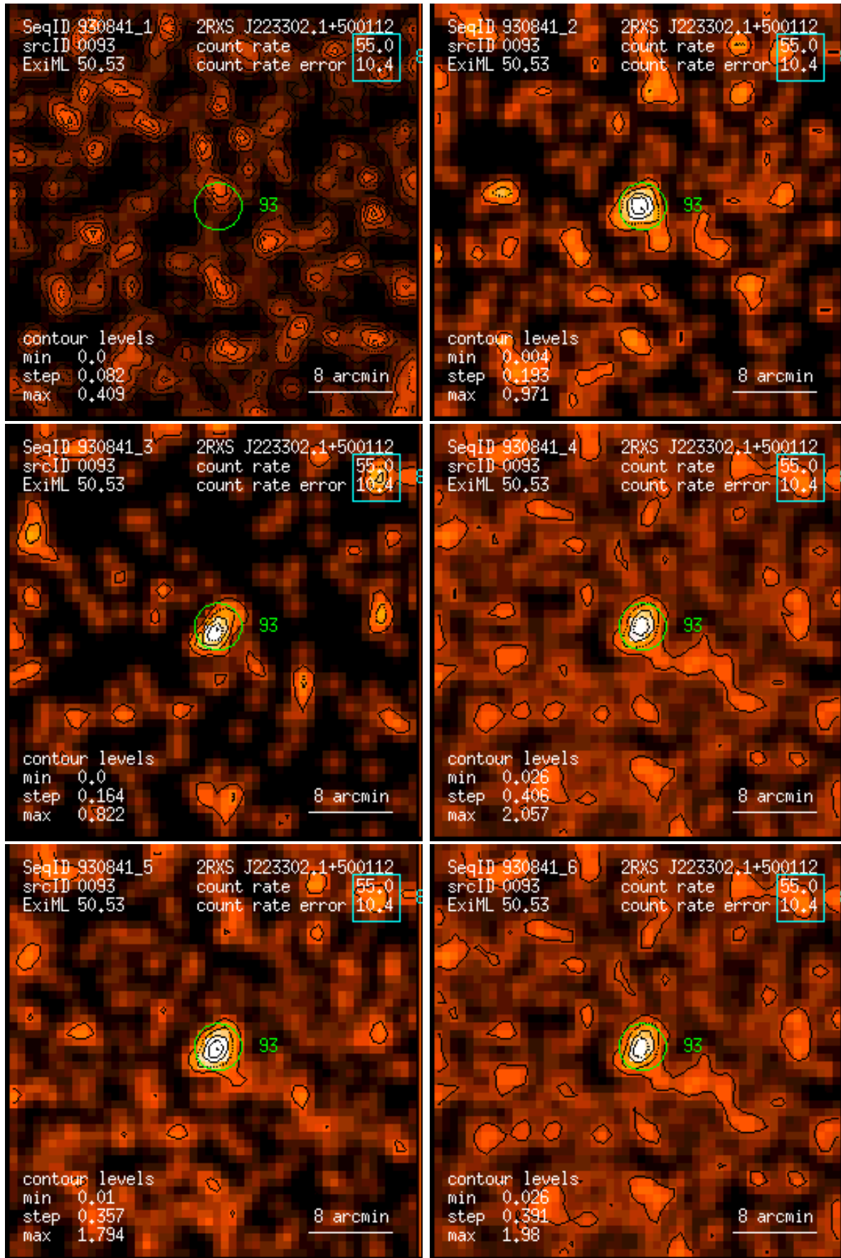
Figure 93: RASS 930841: detection 0093: band rate images, Gaussian filter: (1) PSPC channels 11 – 41, (2) 52 – 90, (3) 91 – 201, (4) 11 – 235, (5) 52 – 201, (6) 11 – 201. Broad band rates in counts/ks. Band rate contour levels in counts/ks/arcmin 2 .
