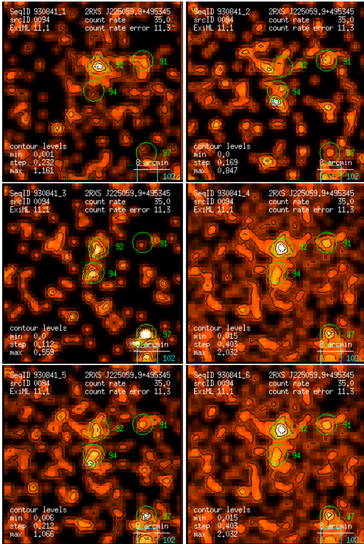
Figure 94: RASS 930841: detection 0094: band rate images, Gaussian filter: (1) PSPC channels 11 – 41, (2) 52 – 90, (3) 91 – 201, (4) 11 – 235, (5) 52 – 201, (6) 11 – 201. Broad band rates in counts/ks. Band rate contour levels in counts/ks/arcmin 2 .
