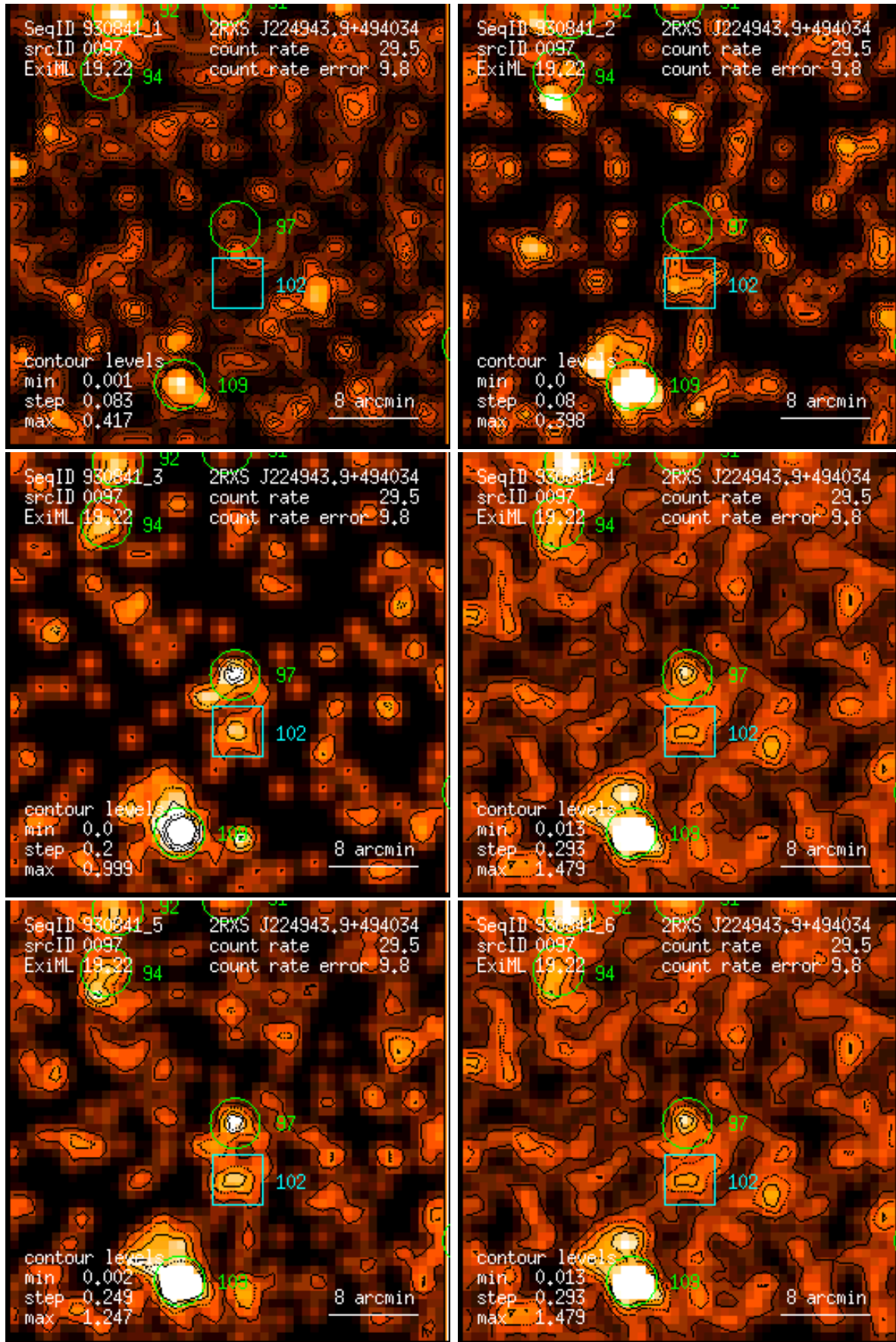
Figure 97: RASS 930841: detection 0097: band rate images, Gaussian filter: (1) PSPC channels 11 – 41, (2) 52 – 90, (3) 91 – 201, (4) 11 – 235, (5) 52 – 201, (6) 11 – 201. Broad band rates in counts/ks. Band rate contour levels in counts/ks/arcmin 2 .
