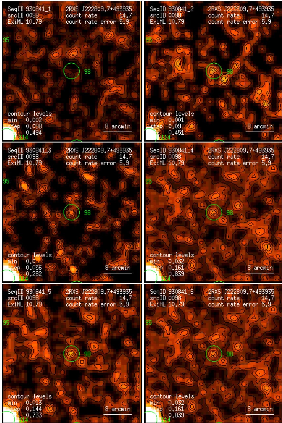
Figure 98: RASS 930841: detection 0098: band rate images, Gaussian filter: (1) PSPC channels 11 – 41, (2) 52 – 90, (3) 91 – 201, (4) 11 – 235, (5) 52 – 201, (6) 11 – 201. Broad band rates in counts/ks. Band rate contour levels in counts/ks/arcmin 2 .
