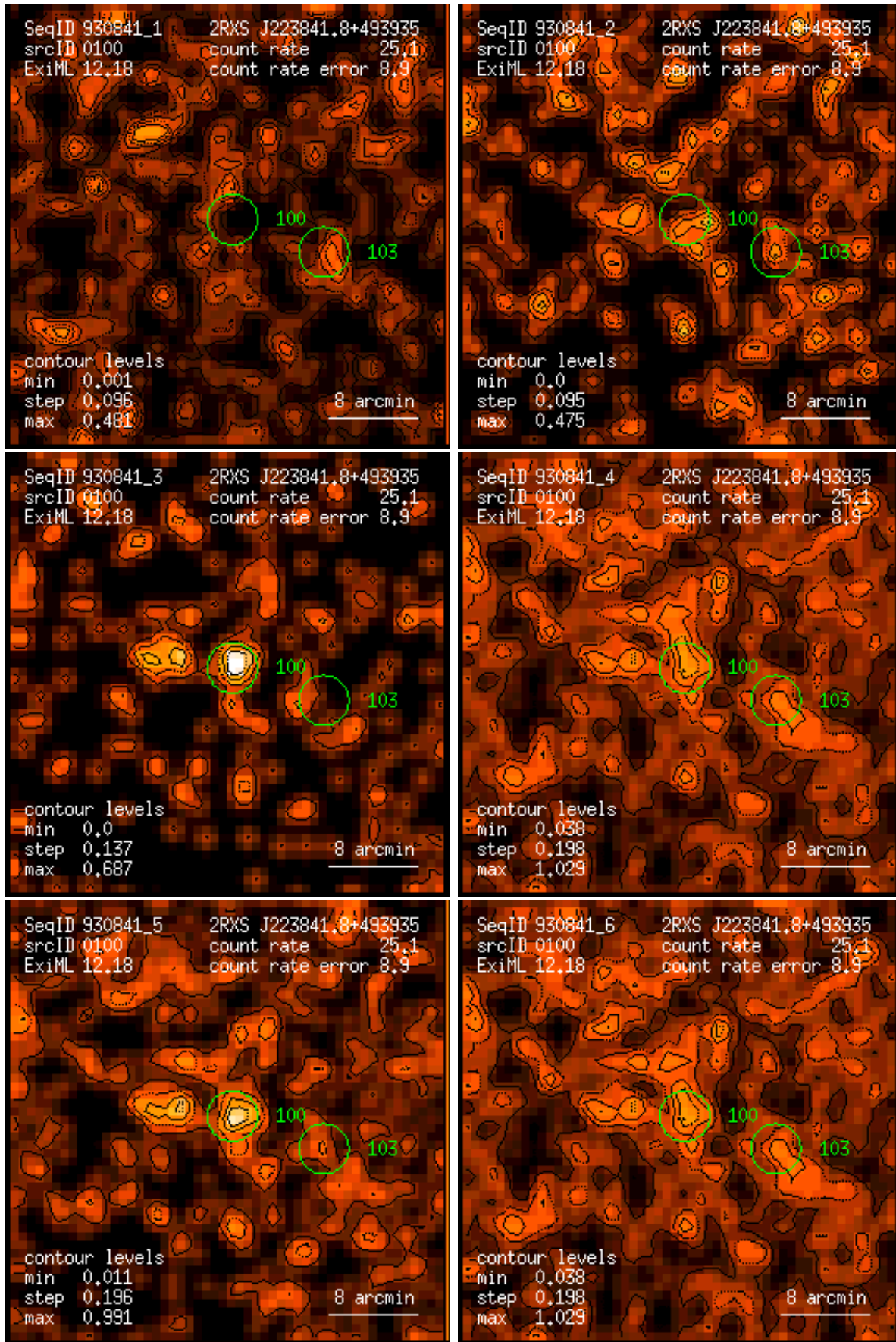
Figure 100: RASS 930841: detection 0100: band rate images, Gaussian filter: (1) PSPC channels 11 – 41, (2) 52 – 90, (3) 91 – 201, (4) 11 – 235, (5) 52 – 201, (6) 11 – 201. Broad band rates in counts/ks. Band rate contour levels in counts/ks/arcmin 2 .
