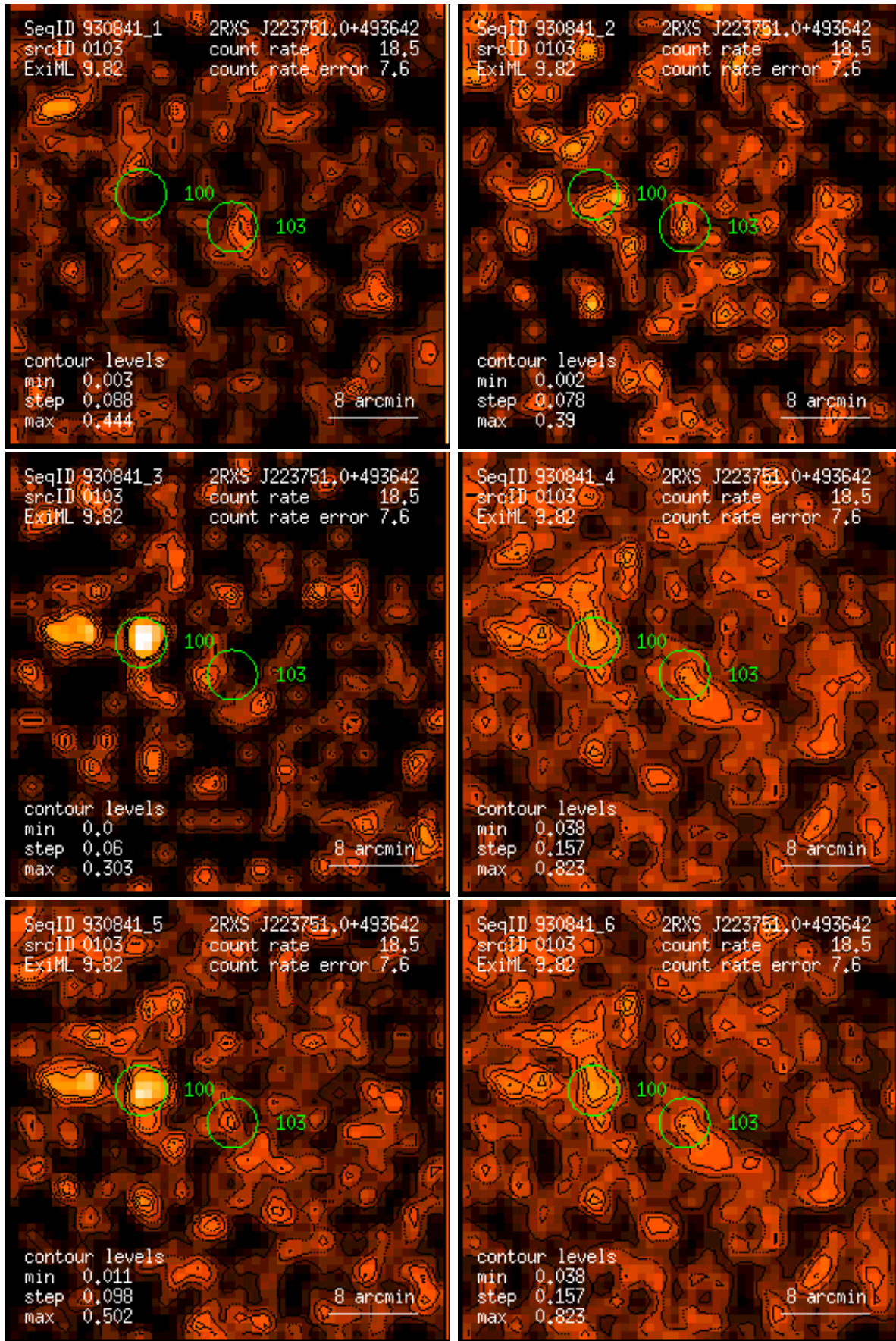
Figure 103: RASS 930841: detection 0103: band rate images, Gaussian filter: (1) PSPC channels 11 – 41, (2) 52 – 90, (3) 91 – 201, (4) 11 – 235, (5) 52 – 201, (6) 11 – 201. Broad band rates in counts/ks. Band rate contour levels in counts/ks/arcmin 2 .
