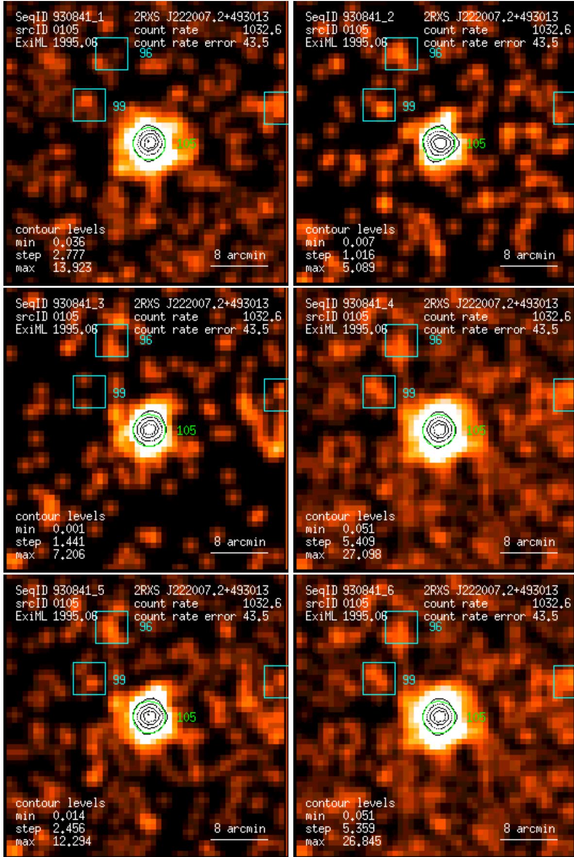
Figure 105: RASS 930841: detection 0105: band rate images, Gaussian filter: (1) PSPC channels 11 – 41, (2) 52 – 90, (3) 91 – 201, (4) 11 – 235, (5) 52 – 201, (6) 11 – 201. Broad band rates in counts/ks. Band rate contour levels in counts/ks/arcmin 2 .
