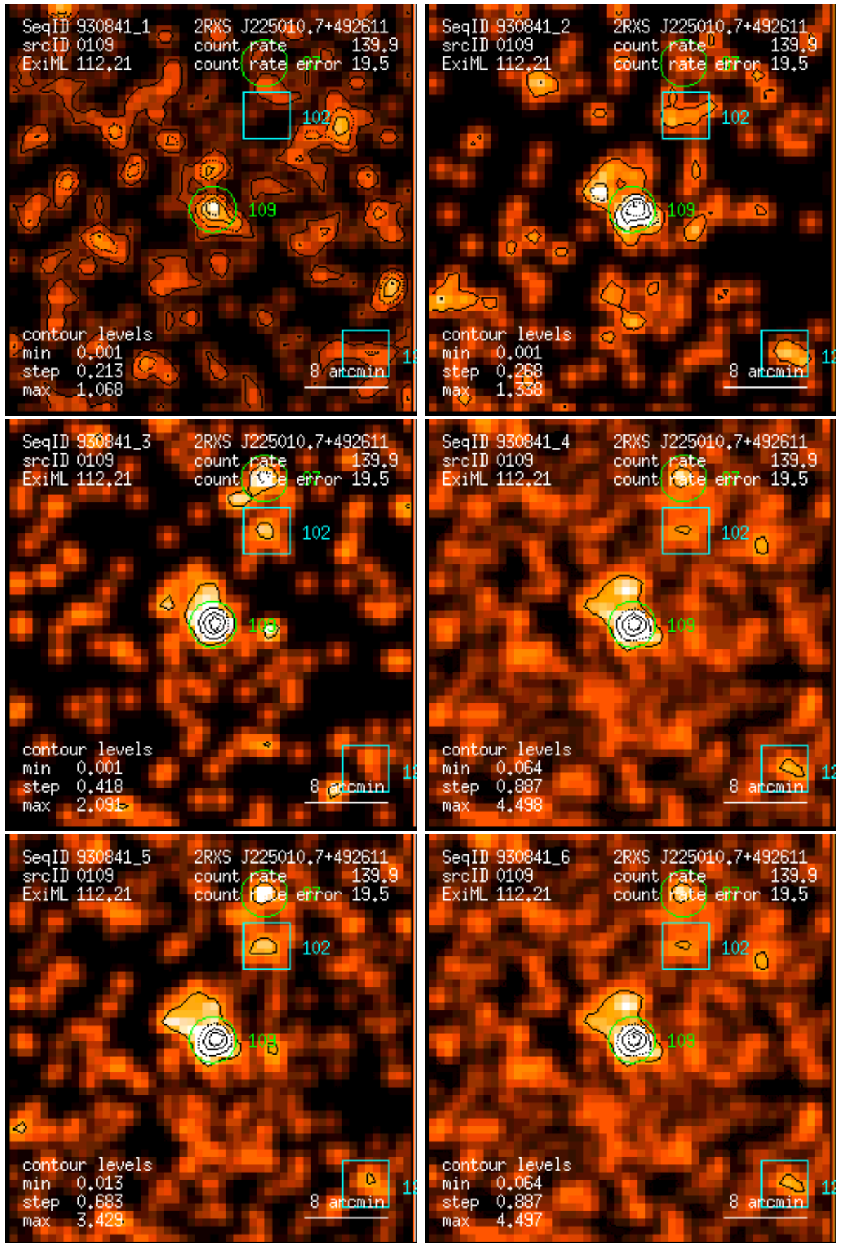
Figure 109: RASS 930841: detection 0109: band rate images, Gaussian filter: (1) PSPC channels 11 – 41, (2) 52 – 90, (3) 91 – 201, (4) 11 – 235, (5) 52 – 201, (6) 11 – 201. Broad band rates in counts/ks. Band rate contour levels in counts/ks/arcmin 2 .
