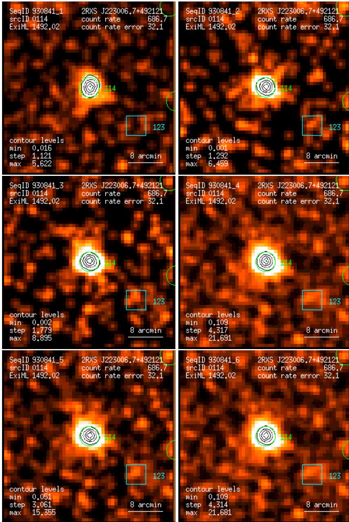
Figure 114: RASS 930841: detection 0114: band rate images, Gaussian filter: (1) PSPC channels 11 – 41, (2) 52 – 90, (3) 91 – 201, (4) 11 – 235, (5) 52 – 201, (6) 11 – 201. Broad band rates in counts/ks. Band rate contour levels in counts/ks/arcmin 2 .
