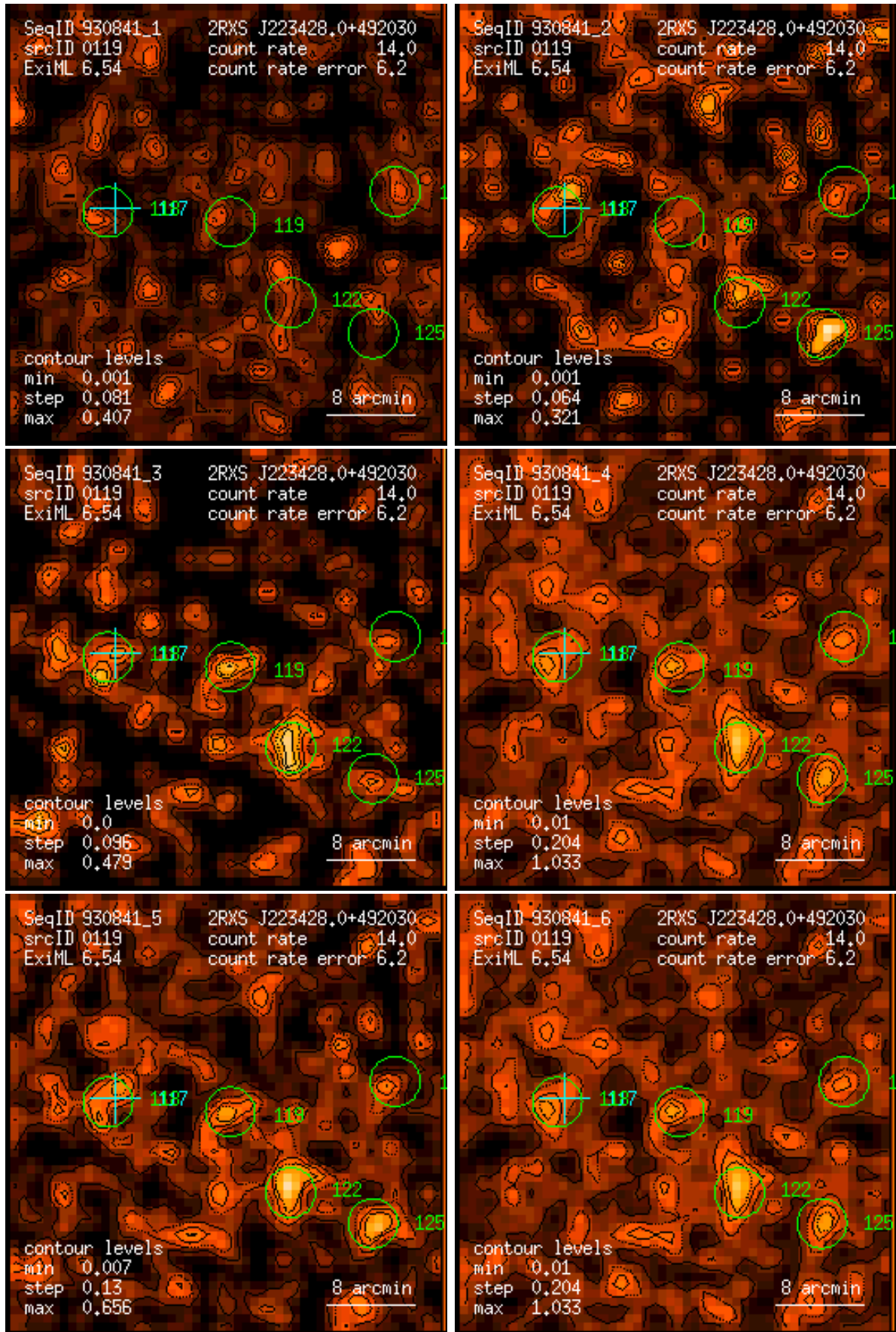
Figure 119: RASS 930841: detection 0119: band rate images, Gaussian filter: (1) PSPC channels 11 – 41, (2) 52 – 90, (3) 91 – 201, (4) 11 – 235, (5) 52 – 201, (6) 11 – 201. Broad band rates in counts/ks. Band rate contour levels in counts/ks/arcmin 2 .
