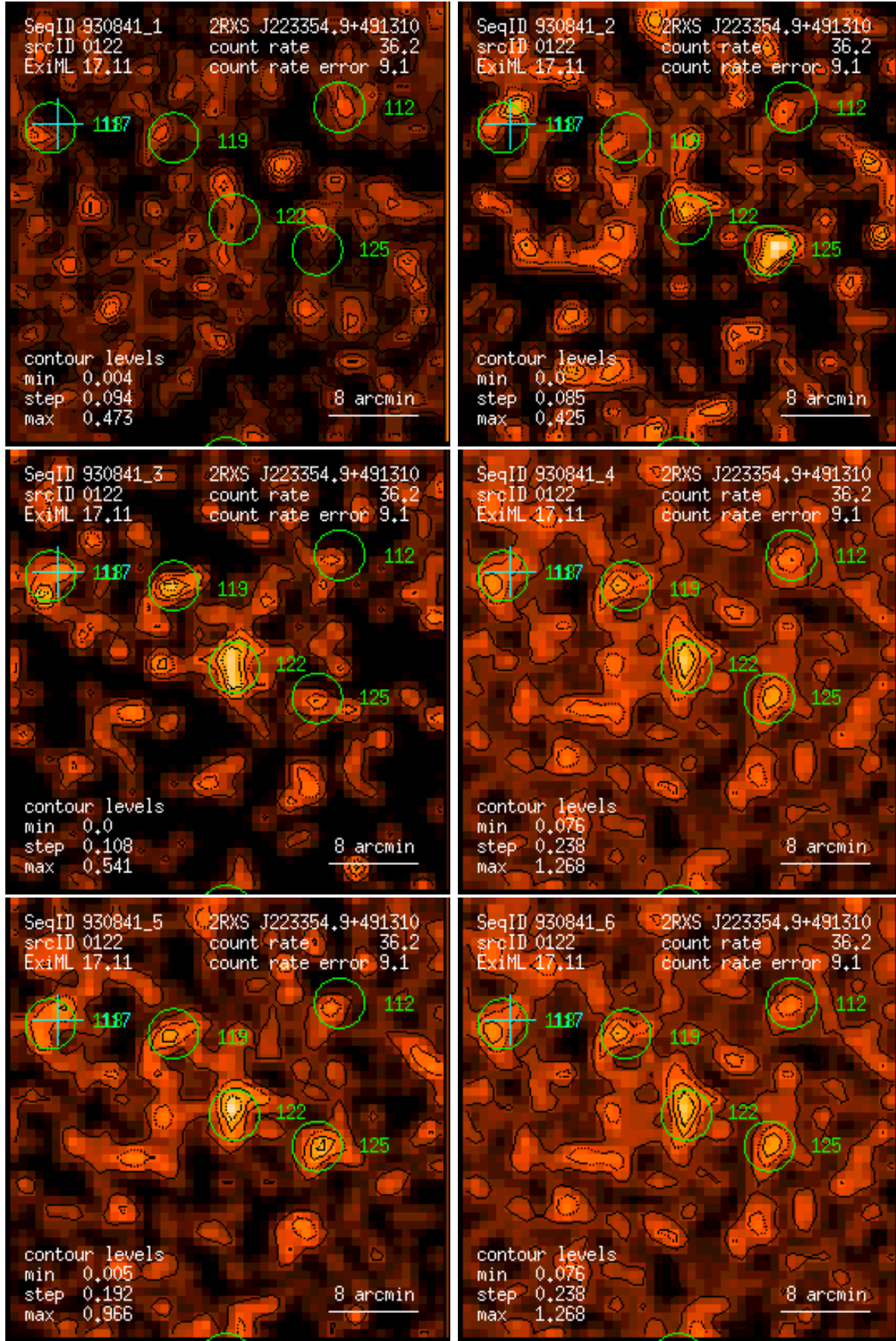
Figure 122: RASS 930841: detection 0122: band rate images, Gaussian filter: (1) PSPC channels 11 – 41, (2) 52 – 90, (3) 91 – 201, (4) 11 – 235, (5) 52 – 201, (6) 11 – 201. Broad band rates in counts/ks. Band rate contour levels in counts/ks/arcmin 2 .
