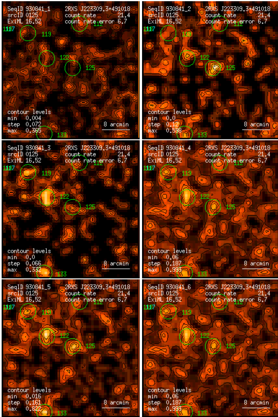
Figure 125: RASS 930841: detection 0125: band rate images, Gaussian filter: (1) PSPC channels 11 – 41, (2) 52 – 90, (3) 91 – 201, (4) 11 – 235, (5) 52 – 201, (6) 11 – 201. Broad band rates in counts/ks. Band rate contour levels in counts/ks/arcmin 2 .
