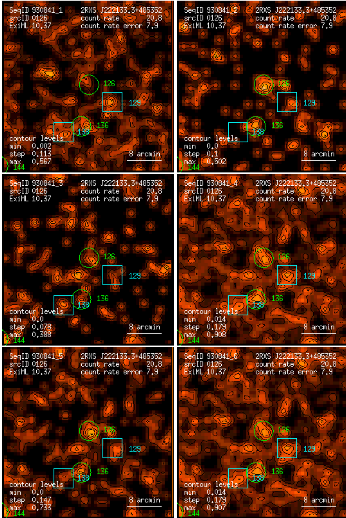
Figure 126: RASS 930841: detection 0126: band rate images, Gaussian filter: (1) PSPC channels 11 – 41, (2) 52 – 90, (3) 91 – 201, (4) 11 – 235, (5) 52 – 201, (6) 11 – 201. Broad band rates in counts/ks. Band rate contour levels in counts/ks/arcmin 2 .
