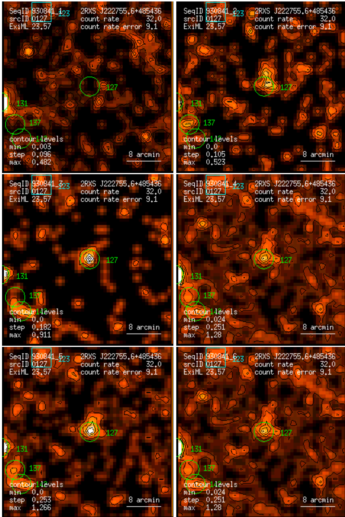
Figure 127: RASS 930841: detection 0127: band rate images, Gaussian filter: (1) PSPC channels 11 – 41, (2) 52 – 90, (3) 91 – 201, (4) 11 – 235, (5) 52 – 201, (6) 11 – 201. Broad band rates in counts/ks. Band rate contour levels in counts/ks/arcmin 2 .
