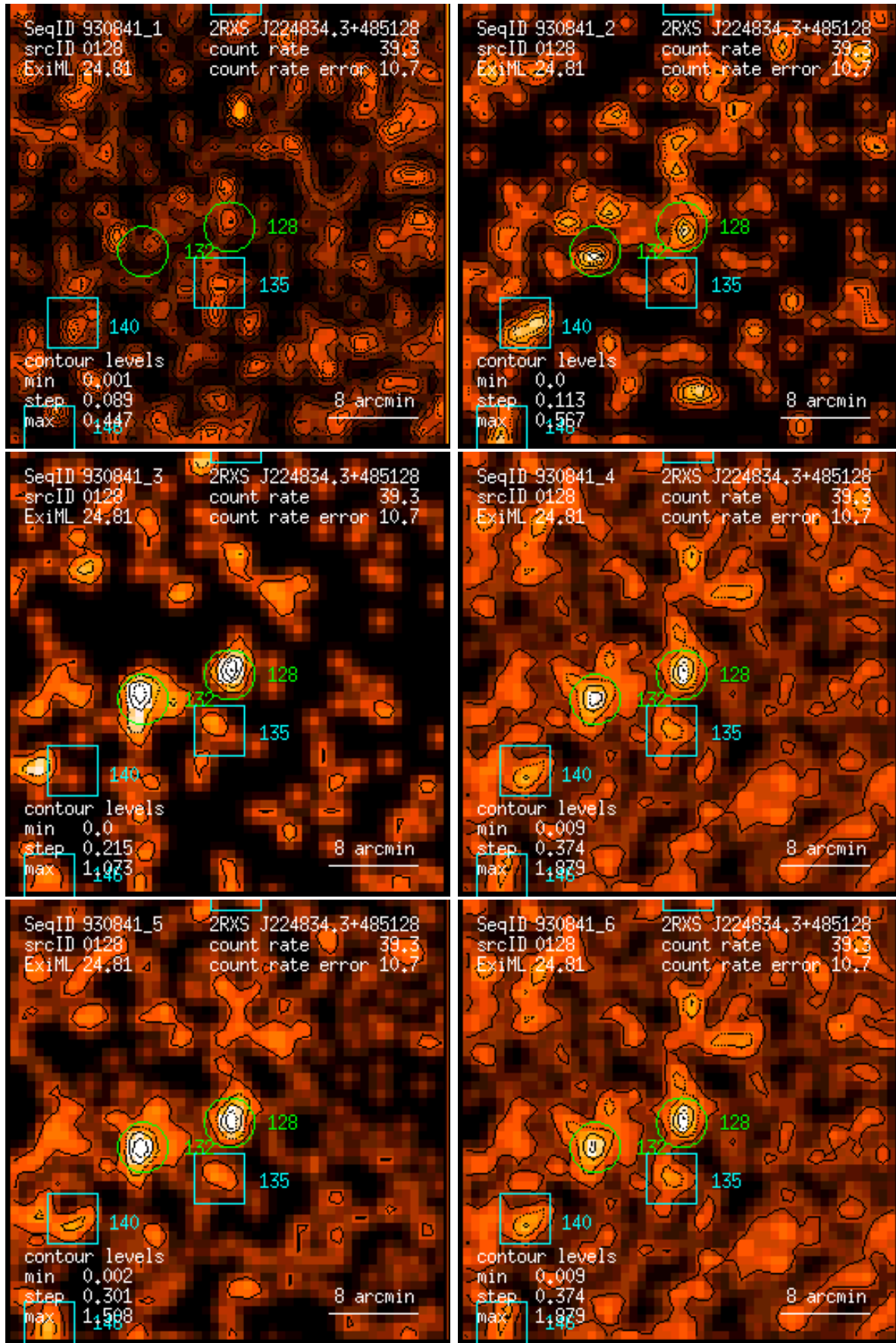
Figure 128: RASS 930841: detection 0128: band rate images, Gaussian filter: (1) PSPC channels 11 – 41, (2) 52 – 90, (3) 91 – 201, (4) 11 – 235, (5) 52 – 201, (6) 11 – 201. Broad band rates in counts/ks. Band rate contour levels in counts/ks/arcmin 2 .
