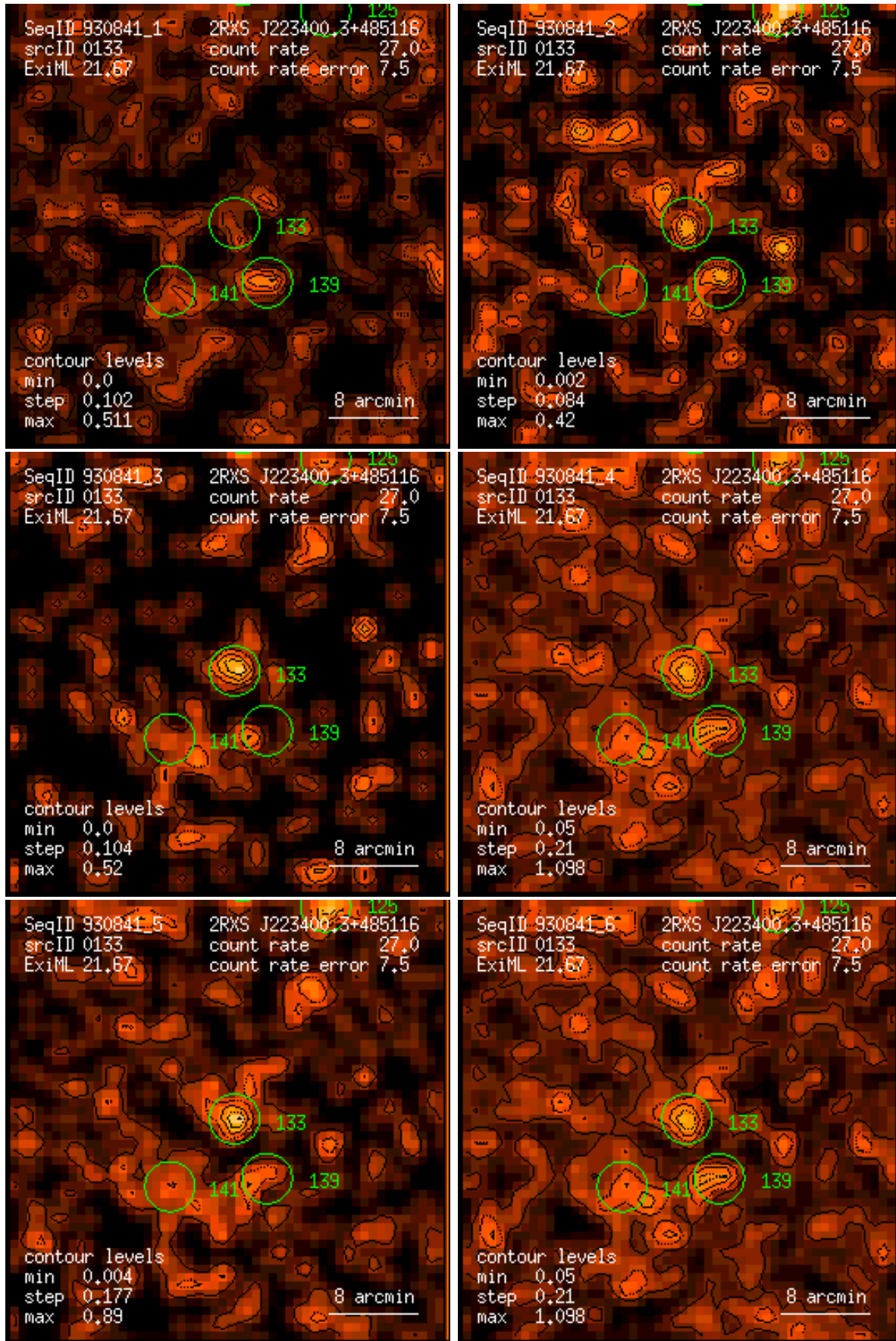
Figure 133: RASS 930841: detection 0133: band rate images, Gaussian filter: (1) PSPC channels 11 – 41, (2) 52 – 90, (3) 91 – 201, (4) 11 – 235, (5) 52 – 201, (6) 11 – 201. Broad band rates in counts/ks. Band rate contour levels in counts/ks/arcmin 2 .
