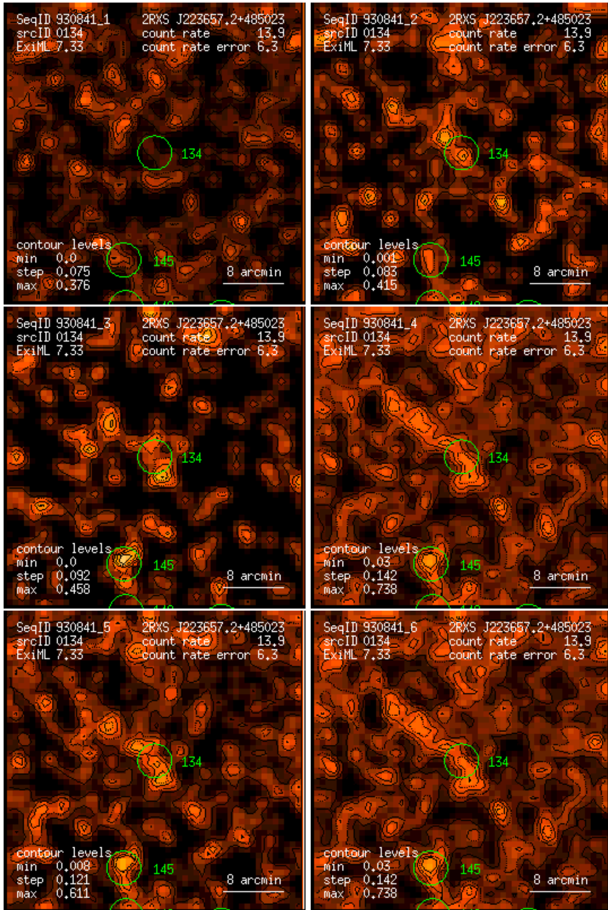
Figure 134: RASS 930841: detection 0134: band rate images, Gaussian filter: (1) PSPC channels 11 – 41, (2) 52 – 90, (3) 91 – 201, (4) 11 – 235, (5) 52 – 201, (6) 11 – 201. Broad band rates in counts/ks. Band rate contour levels in counts/ks/arcmin 2 .
