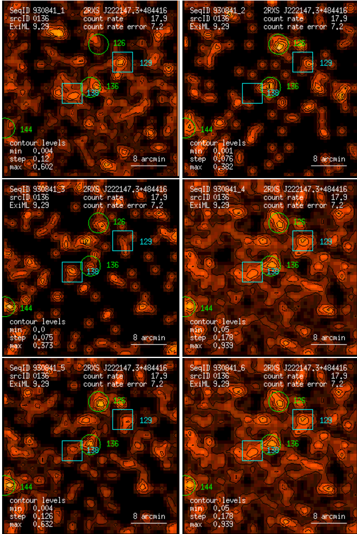
Figure 136: RASS 930841: detection 0136: band rate images, Gaussian filter: (1) PSPC channels 11 – 41, (2) 52 – 90, (3) 91 – 201, (4) 11 – 235, (5) 52 – 201, (6) 11 – 201. Broad band rates in counts/ks. Band rate contour levels in counts/ks/arcmin 2 .
