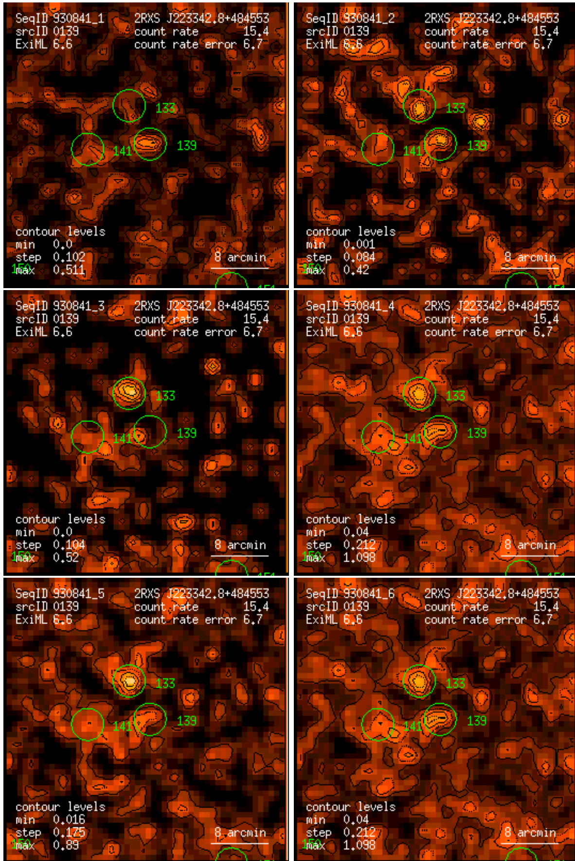
Figure 139: RASS 930841: detection 0139: band rate images, Gaussian filter: (1) PSPC channels 11 – 41, (2) 52 – 90, (3) 91 – 201, (4) 11 – 235, (5) 52 – 201, (6) 11 – 201. Broad band rates in counts/ks. Band rate contour levels in counts/ks/arcmin 2 .
