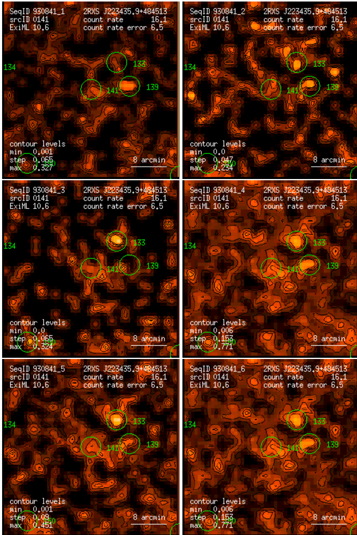
Figure 141: RASS 930841: detection 0141: band rate images, Gaussian filter: (1) PSPC channels 11 – 41, (2) 52 – 90, (3) 91 – 201, (4) 11 – 235, (5) 52 – 201, (6) 11 – 201. Broad band rates in counts/ks. Band rate contour levels in counts/ks/arcmin 2 .
