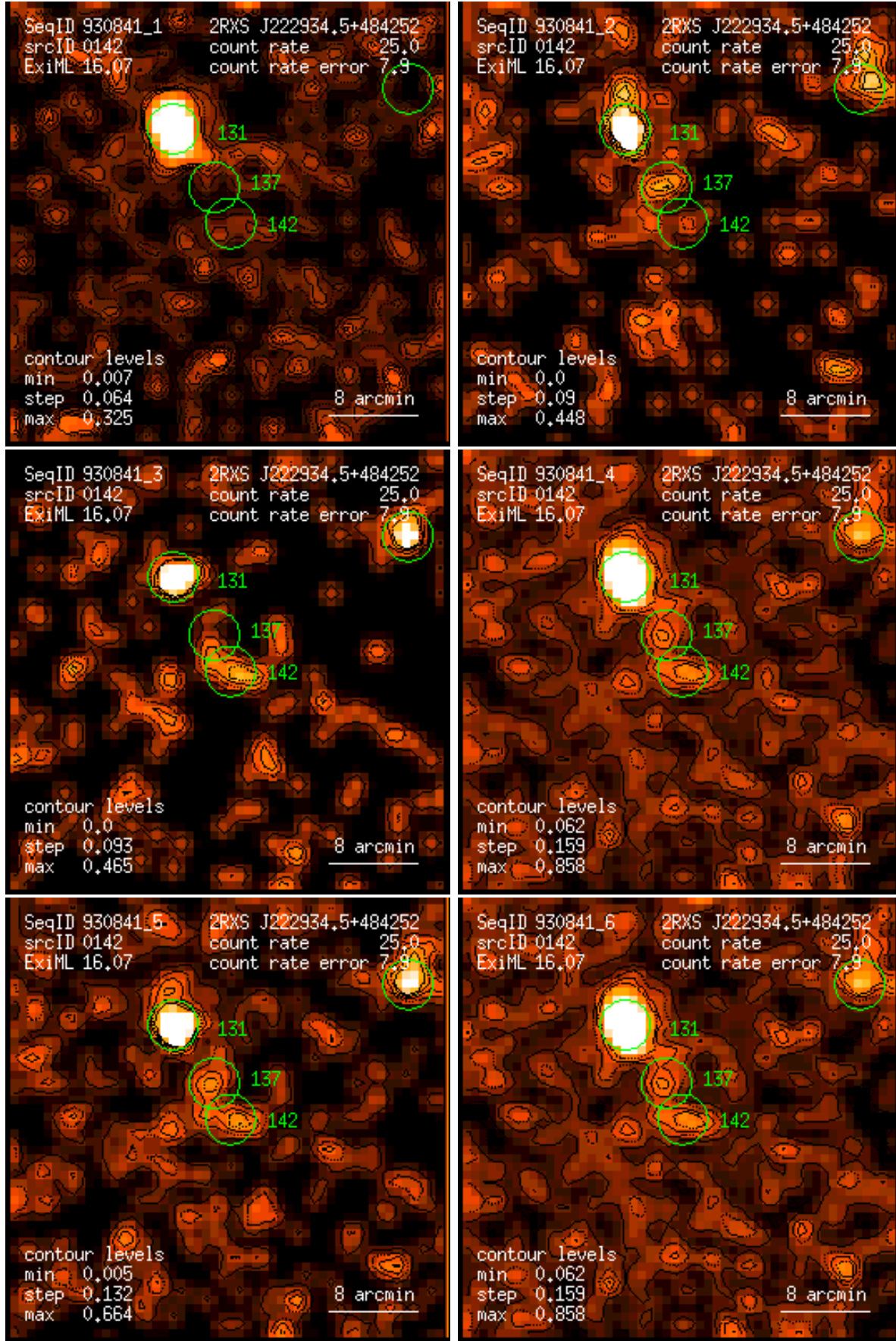
Figure 142: RASS 930841: detection 0142: band rate images, Gaussian filter: (1) PSPC channels 11 – 41, (2) 52 – 90, (3) 91 – 201, (4) 11 – 235, (5) 52 – 201, (6) 11 – 201. Broad band rates in counts/ks. Band rate contour levels in counts/ks/arcmin 2 .
