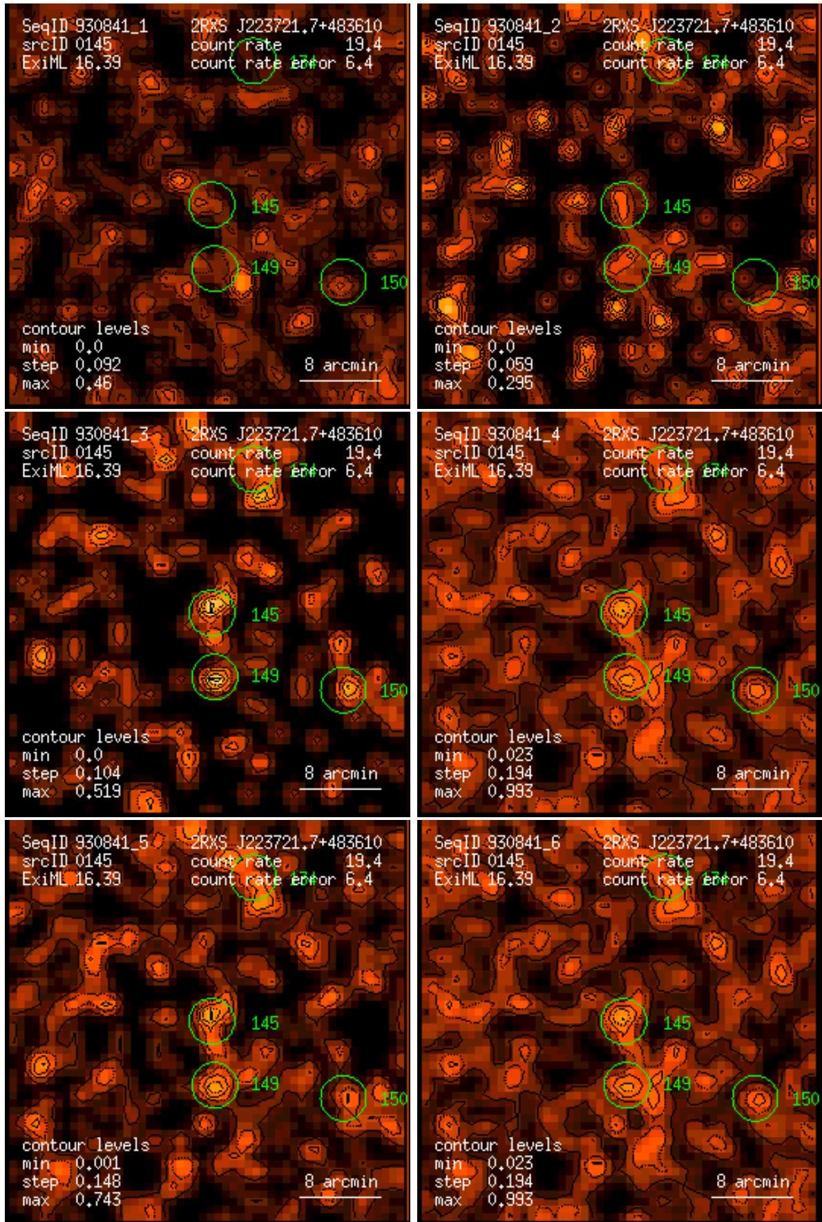
Figure 145: RASS 930841: detection 0145: band rate images, Gaussian filter: (1) PSPC channels 11 – 41, (2) 52 – 90, (3) 91 – 201, (4) 11 – 235, (5) 52 – 201, (6) 11 – 201. Broad band rates in counts/ks. Band rate contour levels in counts/ks/arcmin 2 .
