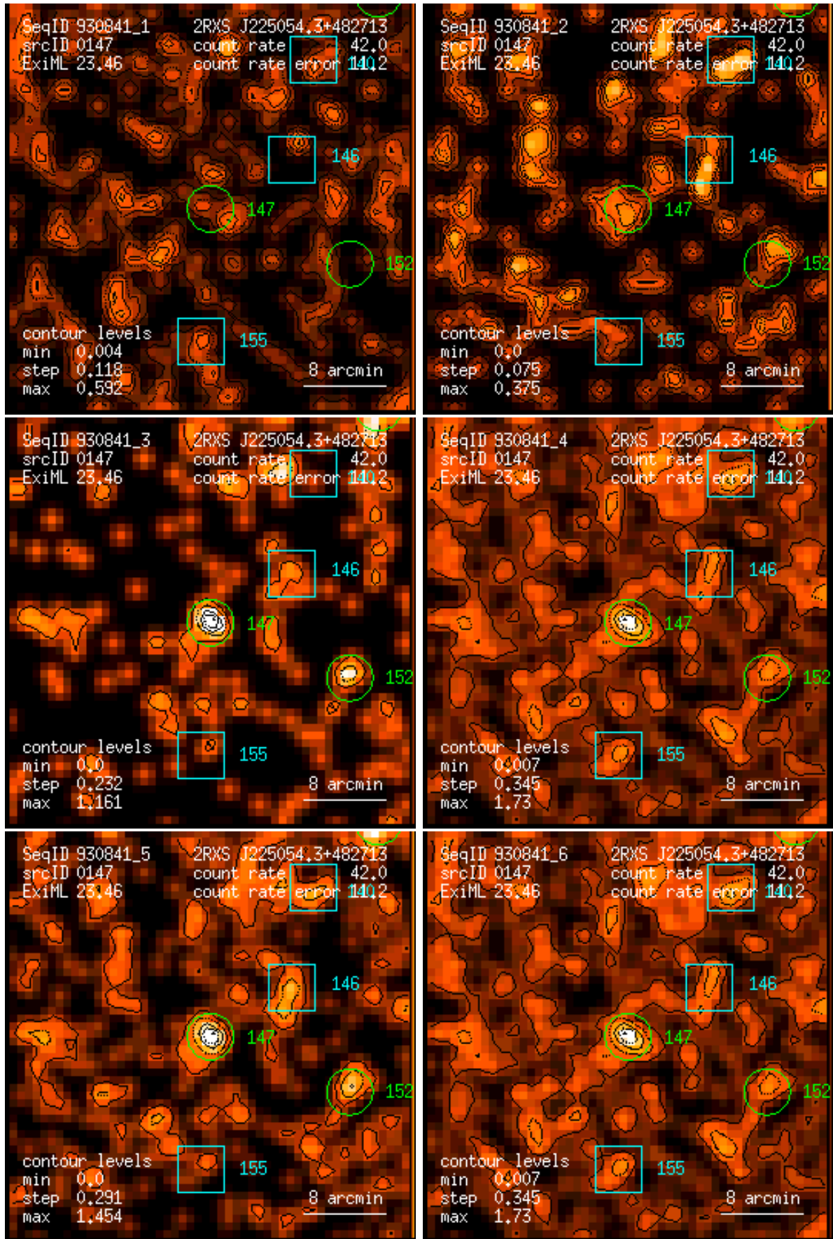
Figure 147: RASS 930841: detection 0147: band rate images, Gaussian filter: (1) PSPC channels 11 – 41, (2) 52 – 90, (3) 91 – 201, (4) 11 – 235, (5) 52 – 201, (6) 11 – 201. Broad band rates in counts/ks. Band rate contour levels in counts/ks/arcmin 2 .
