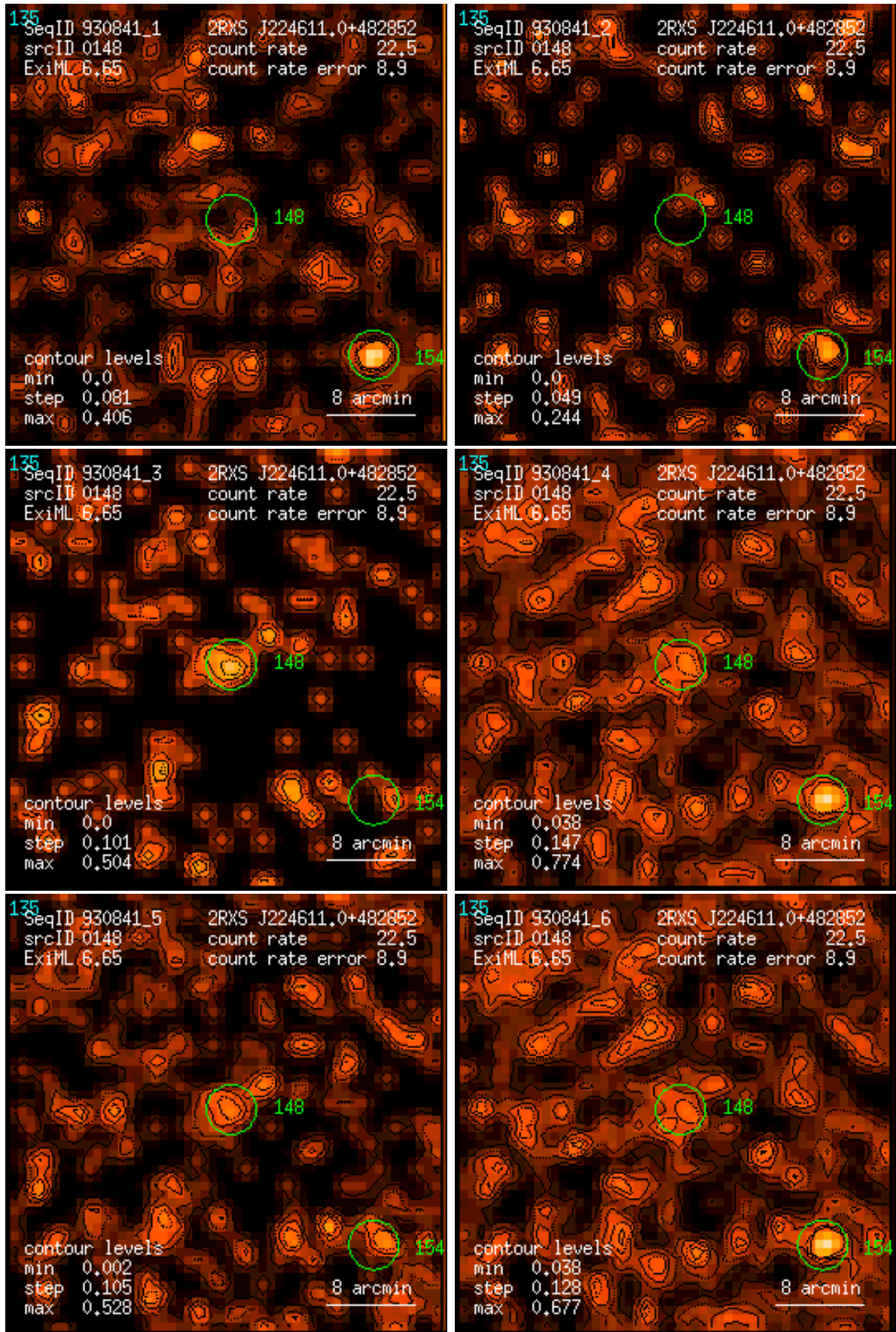
Figure 148: RASS 930841: detection 0148: band rate images, Gaussian filter: (1) PSPC channels 11 – 41, (2) 52 – 90, (3) 91 – 201, (4) 11 – 235, (5) 52 – 201, (6) 11 – 201. Broad band rates in counts/ks. Band rate contour levels in counts/ks/arcmin 2 .
