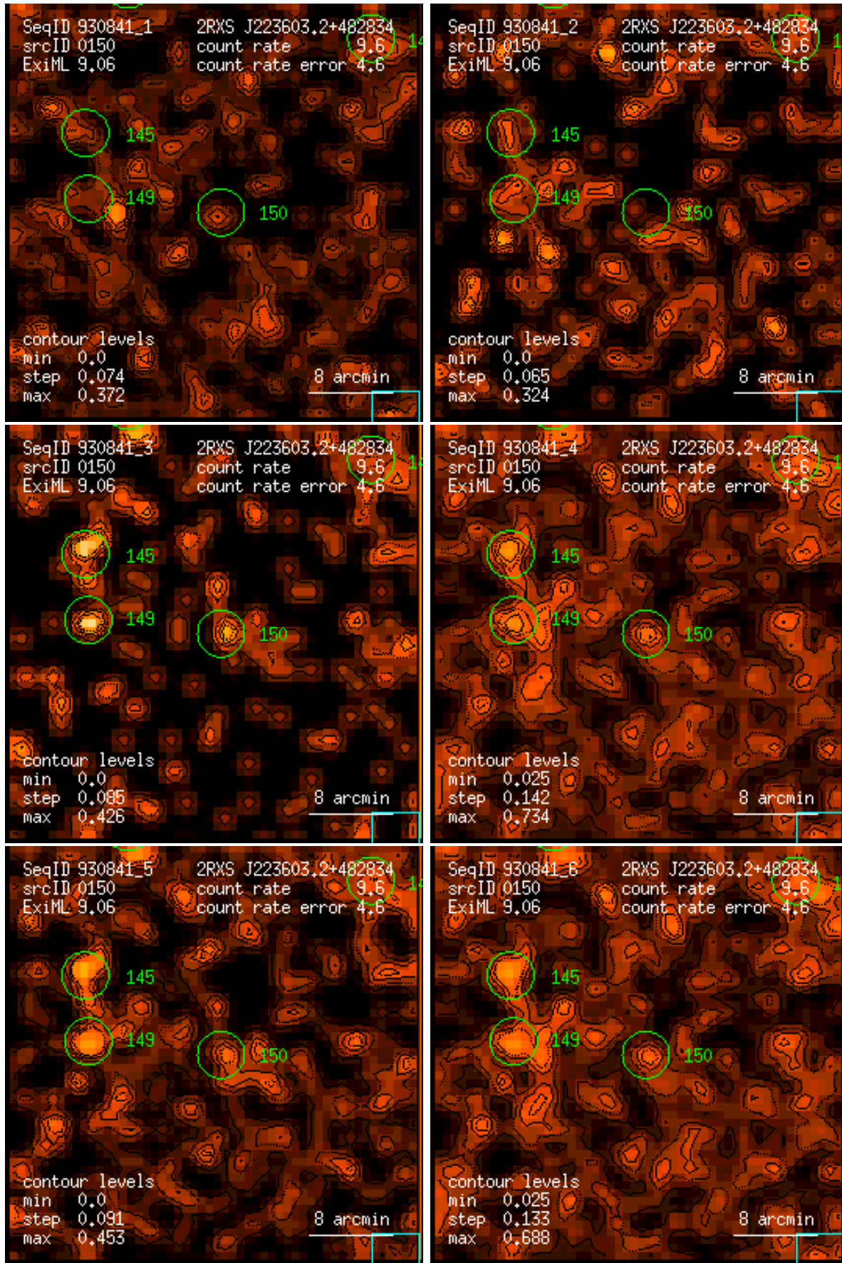
Figure 150: RASS 930841: detection 0150: band rate images, Gaussian filter: (1) PSPC channels 11 – 41, (2) 52 – 90, (3) 91 – 201, (4) 11 – 235, (5) 52 – 201, (6) 11 – 201. Broad band rates in counts/ks. Band rate contour levels in counts/ks/arcmin 2 .
