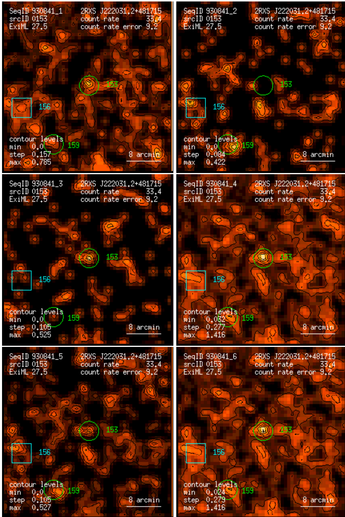
Figure 153: RASS 930841: detection 0153: band rate images, Gaussian filter: (1) PSPC channels 11 – 41, (2) 52 – 90, (3) 91 – 201, (4) 11 – 235, (5) 52 – 201, (6) 11 – 201. Broad band rates in counts/ks. Band rate contour levels in counts/ks/arcmin 2 .
