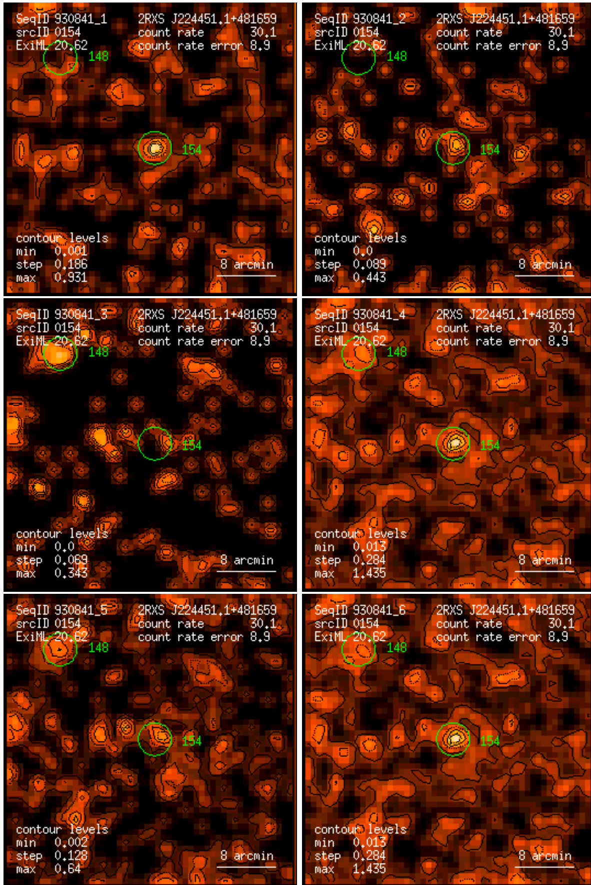
Figure 154: RASS 930841: detection 0154: band rate images, Gaussian filter: (1) PSPC channels 11 – 41, (2) 52 – 90, (3) 91 – 201, (4) 11 – 235, (5) 52 – 201, (6) 11 – 201. Broad band rates in counts/ks. Band rate contour levels in counts/ks/arcmin 2 .
