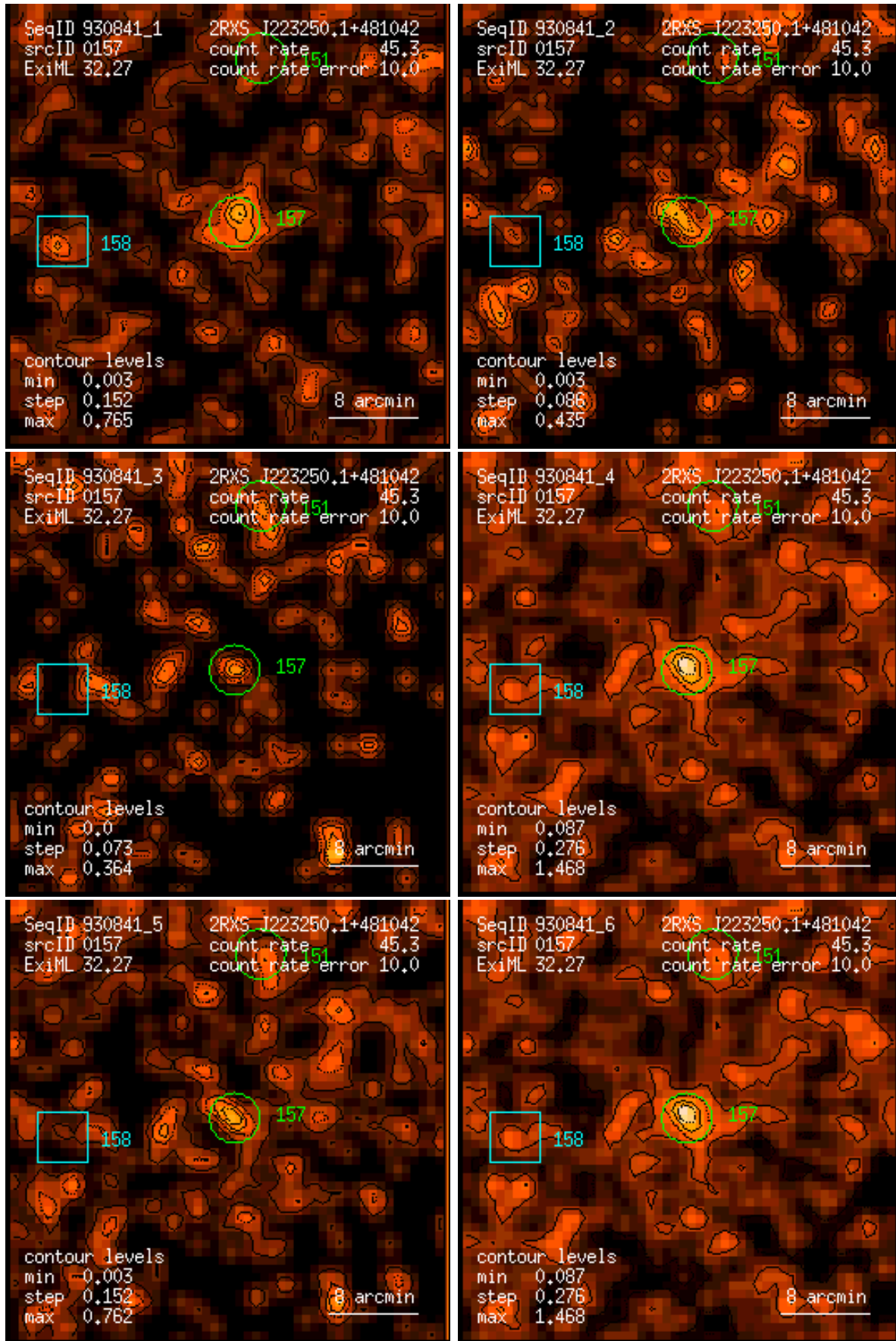
Figure 157: RASS 930841: detection 0157: band rate images, Gaussian filter: (1) PSPC channels 11 – 41, (2) 52 – 90, (3) 91 – 201, (4) 11 – 235, (5) 52 – 201, (6) 11 – 201. Broad band rates in counts/ks. Band rate contour levels in counts/ks/arcmin 2 .
