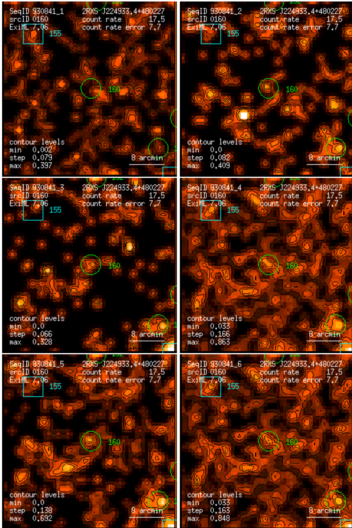
Figure 160: RASS 930841: detection 0160: band rate images, Gaussian filter: (1) PSPC channels 11 – 41, (2) 52 – 90, (3) 91 – 201, (4) 11 – 235, (5) 52 – 201, (6) 11 – 201. Broad band rates in counts/ks. Band rate contour levels in counts/ks/arcmin 2 .
