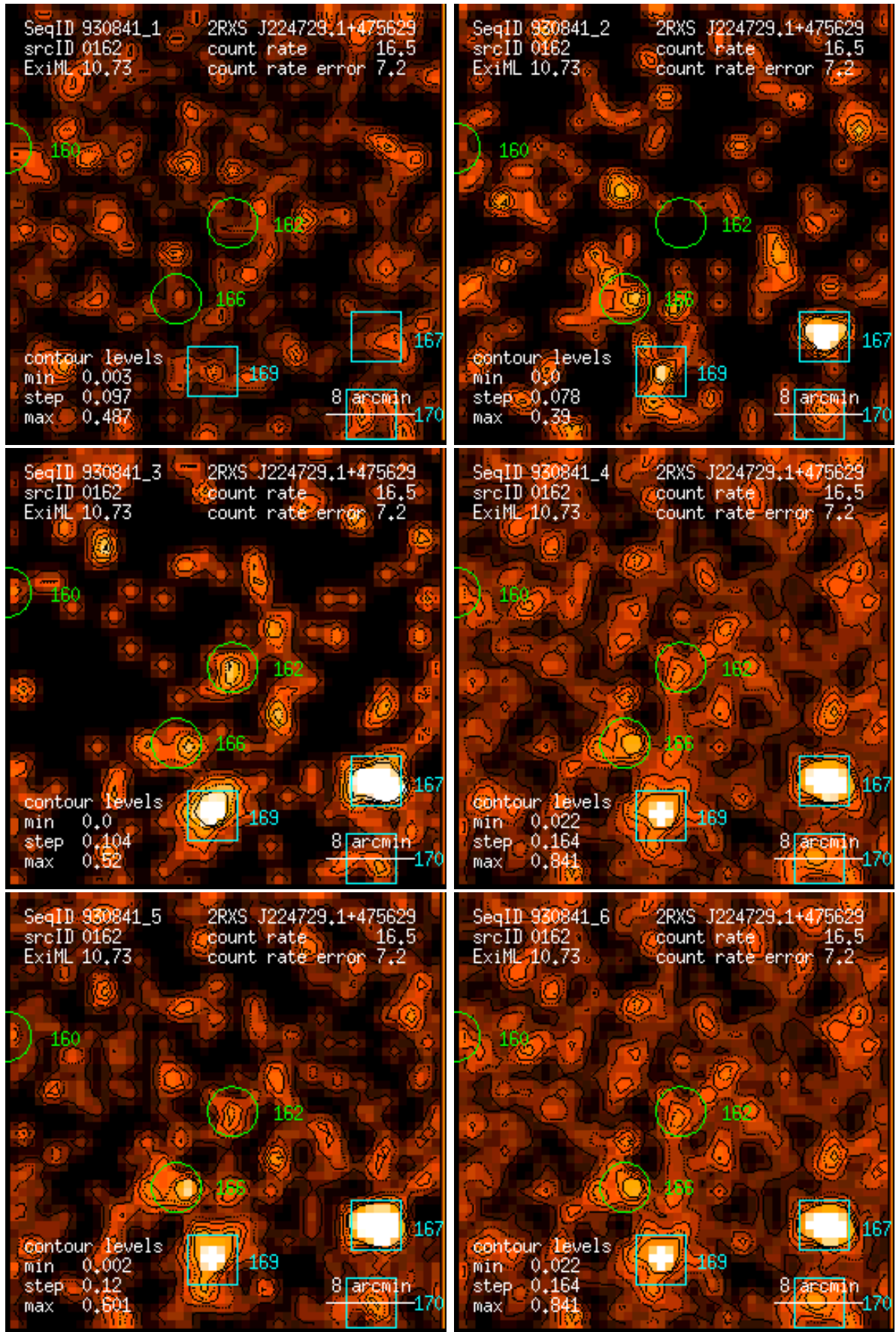
Figure 162: RASS 930841: detection 0162: band rate images, Gaussian filter: (1) PSPC channels 11 – 41, (2) 52 – 90, (3) 91 – 201, (4) 11 – 235, (5) 52 – 201, (6) 11 – 201. Broad band rates in counts/ks. Band rate contour levels in counts/ks/arcmin 2 .
