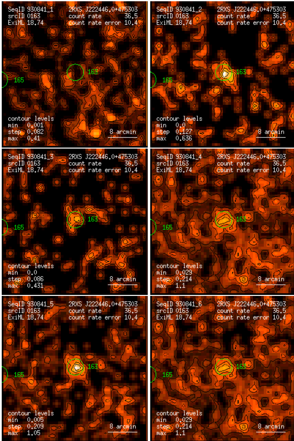
Figure 163: RASS 930841: detection 0163: band rate images, Gaussian filter: (1) PSPC channels 11 – 41, (2) 52 – 90, (3) 91 – 201, (4) 11 – 235, (5) 52 – 201, (6) 11 – 201. Broad band rates in counts/ks. Band rate contour levels in counts/ks/arcmin 2 .
