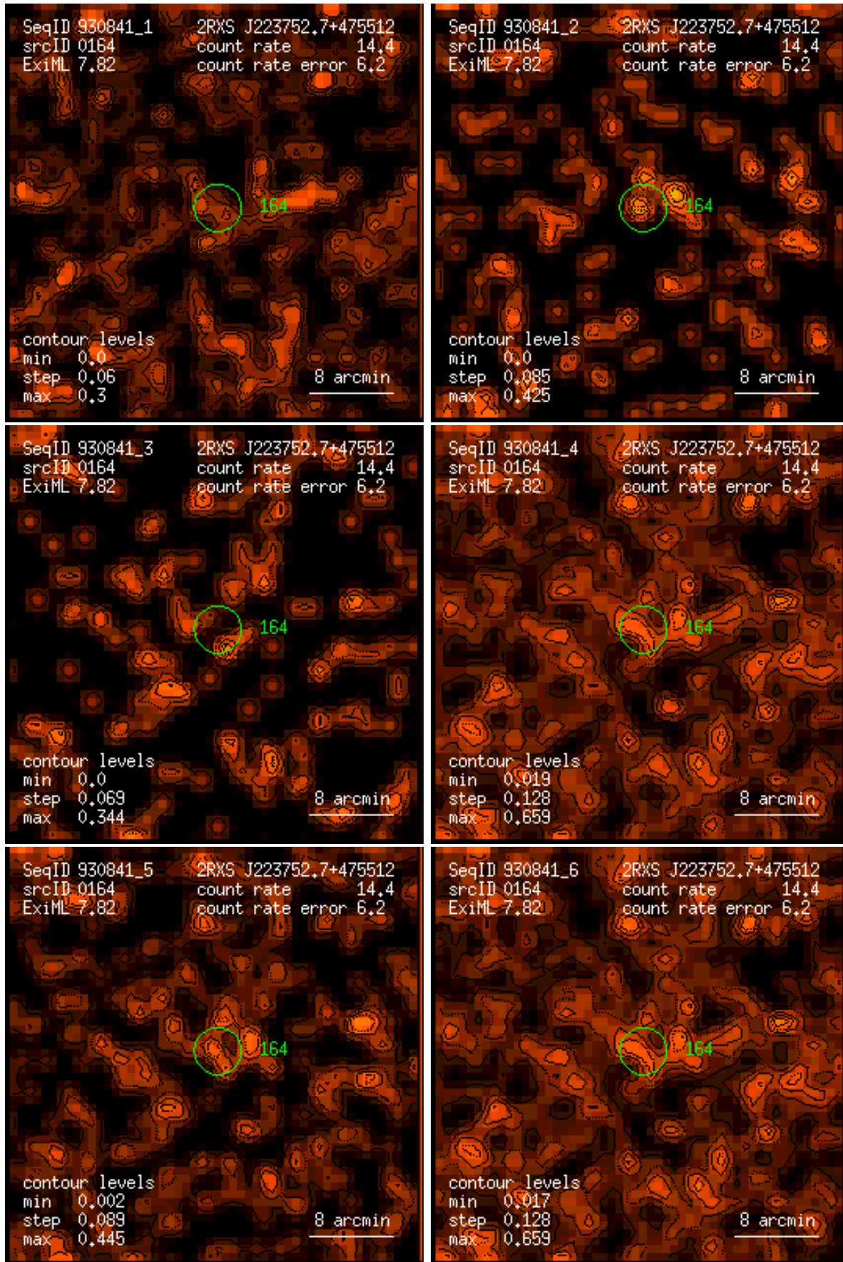
Figure 164: RASS 930841: detection 0164: band rate images, Gaussian filter: (1) PSPC channels 11 – 41, (2) 52 – 90, (3) 91 – 201, (4) 11 – 235, (5) 52 – 201, (6) 11 – 201. Broad band rates in counts/ks. Band rate contour levels in counts/ks/arcmin 2 .
