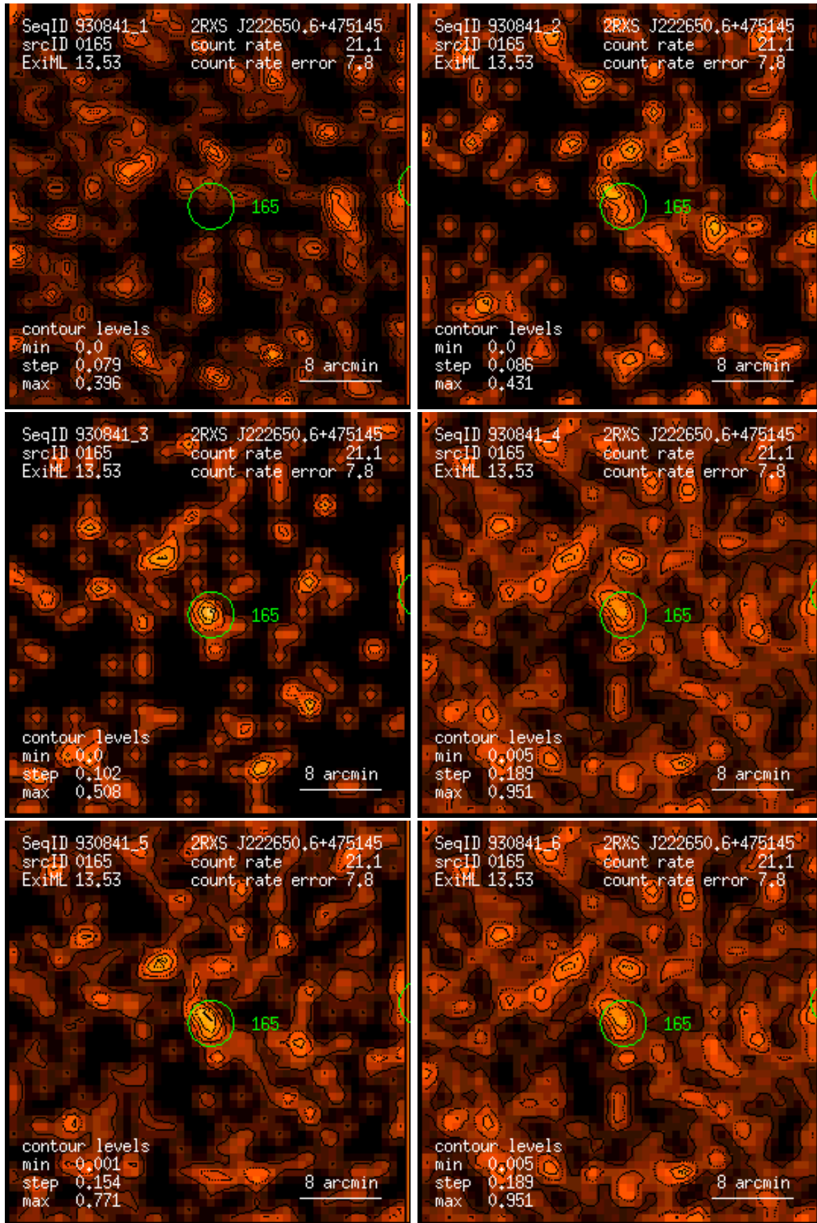
Figure 165: RASS 930841: detection 0165: band rate images, Gaussian filter: (1) PSPC channels 11 – 41, (2) 52 – 90, (3) 91 – 201, (4) 11 – 235, (5) 52 – 201, (6) 11 – 201. Broad band rates in counts/ks. Band rate contour levels in counts/ks/arcmin 2 .
