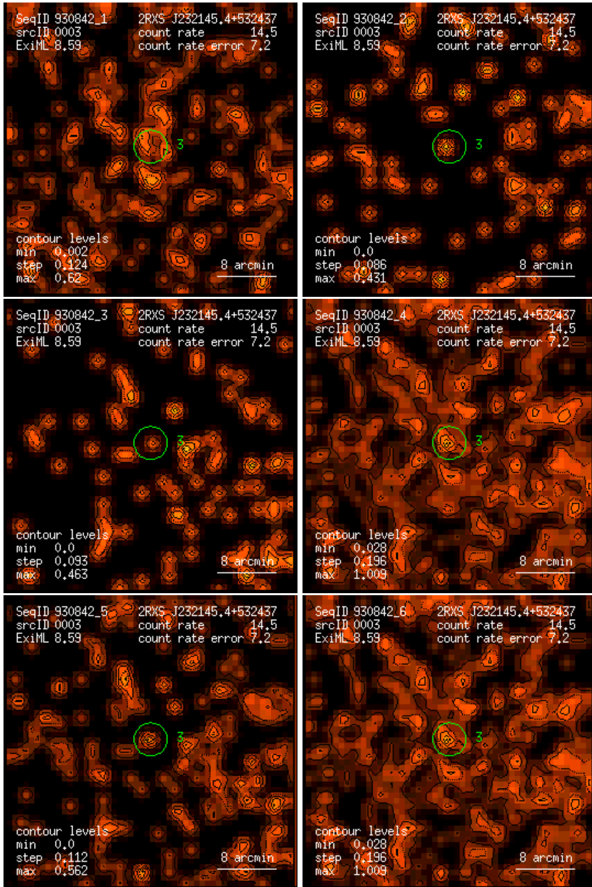
Figure 3: RASS 930842: detection 0003: band rate images, Gaussian filter: (1) PSPC channels 11 – 41, (2) 52 – 90, (3) 91 – 201, (4) 11 – 235, (5) 52 – 201, (6) 11 – 201. Broad band rates in counts/ks. Band rate contour levels in counts/ks/arcmin 2 .
