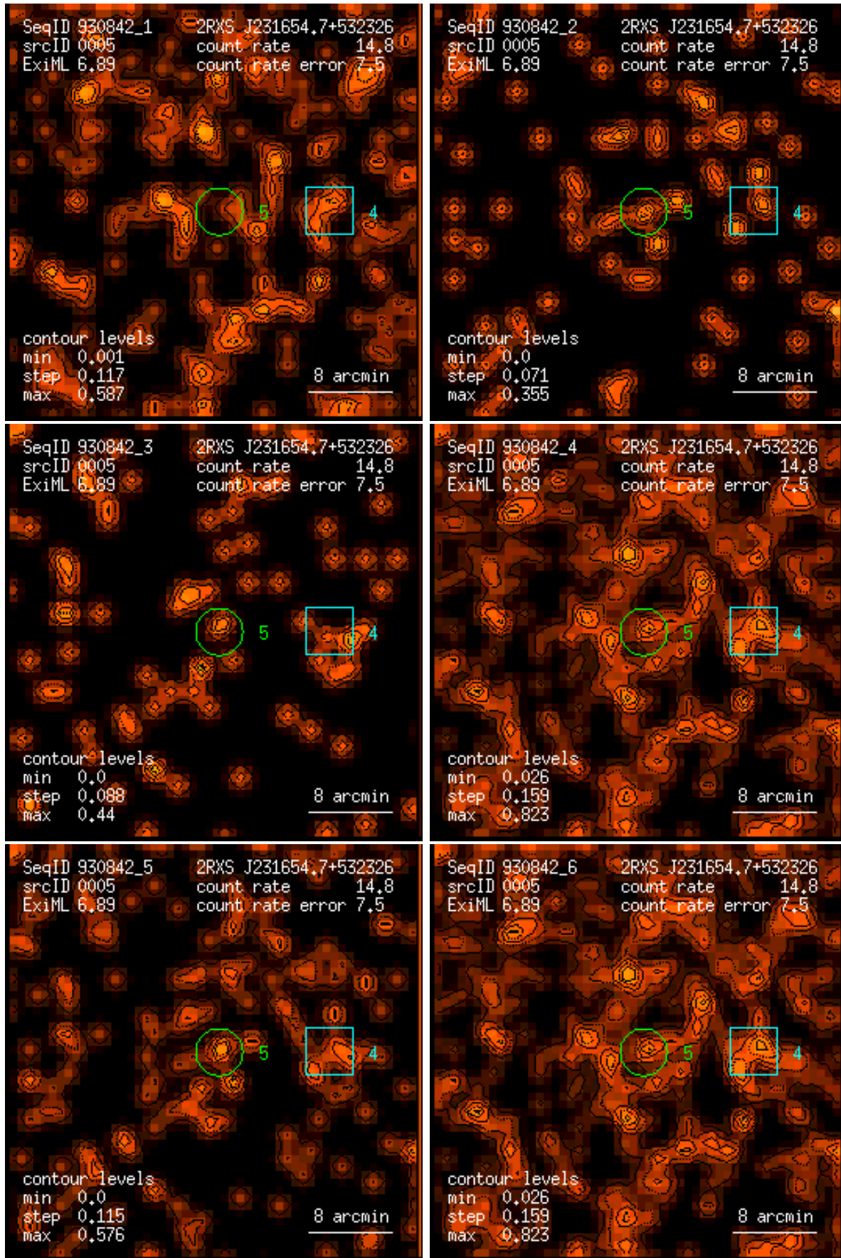
Figure 5: RASS 930842: detection 0005: band rate images, Gaussian filter: (1) PSPC channels 11 – 41, (2) 52 – 90, (3) 91 – 201, (4) 11 – 235, (5) 52 – 201, (6) 11 – 201. Broad band rates in counts/ks. Band rate contour levels in counts/ks/arcmin 2 .
