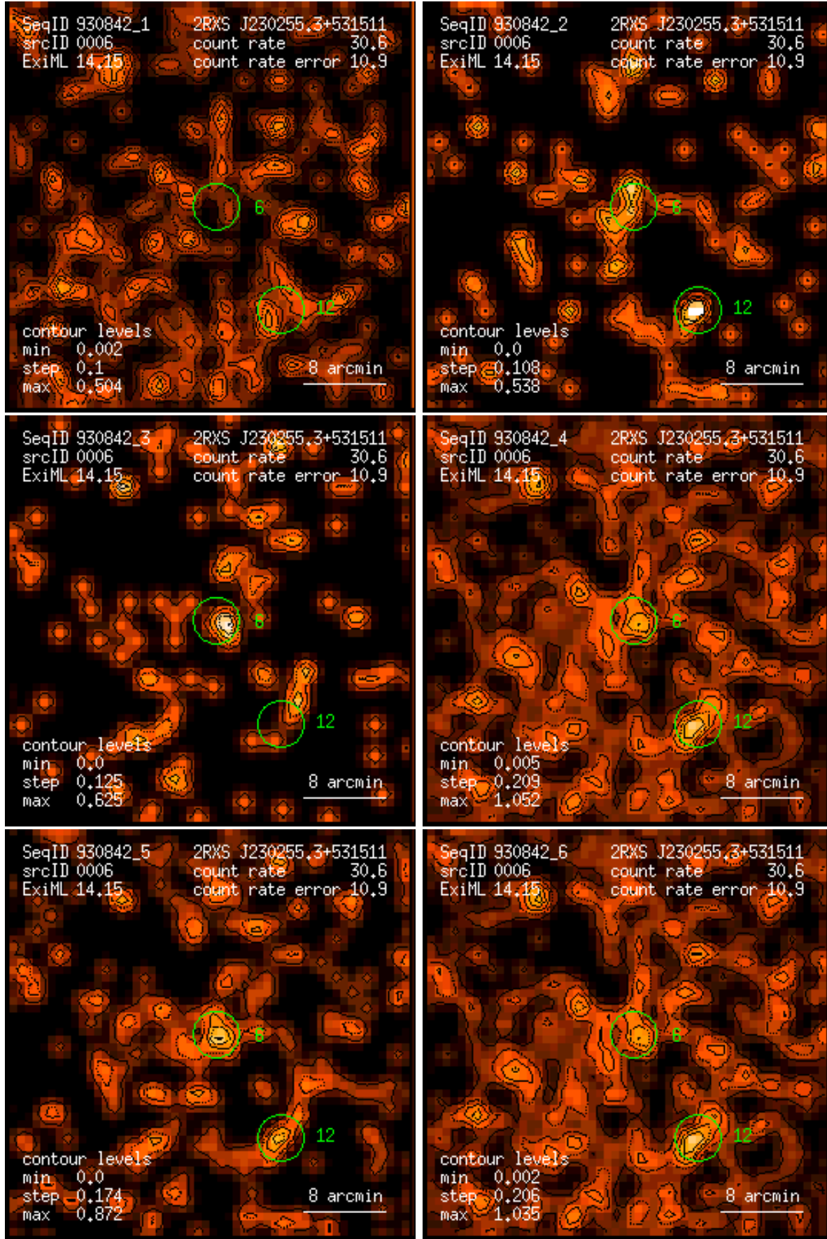
Figure 6: RASS 930842: detection 0006: band rate images, Gaussian filter: (1) PSPC channels 11 – 41, (2) 52 – 90, (3) 91 – 201, (4) 11 – 235, (5) 52 – 201, (6) 11 – 201. Broad band rates in counts/ks. Band rate contour levels in counts/ks/arcmin 2 .
