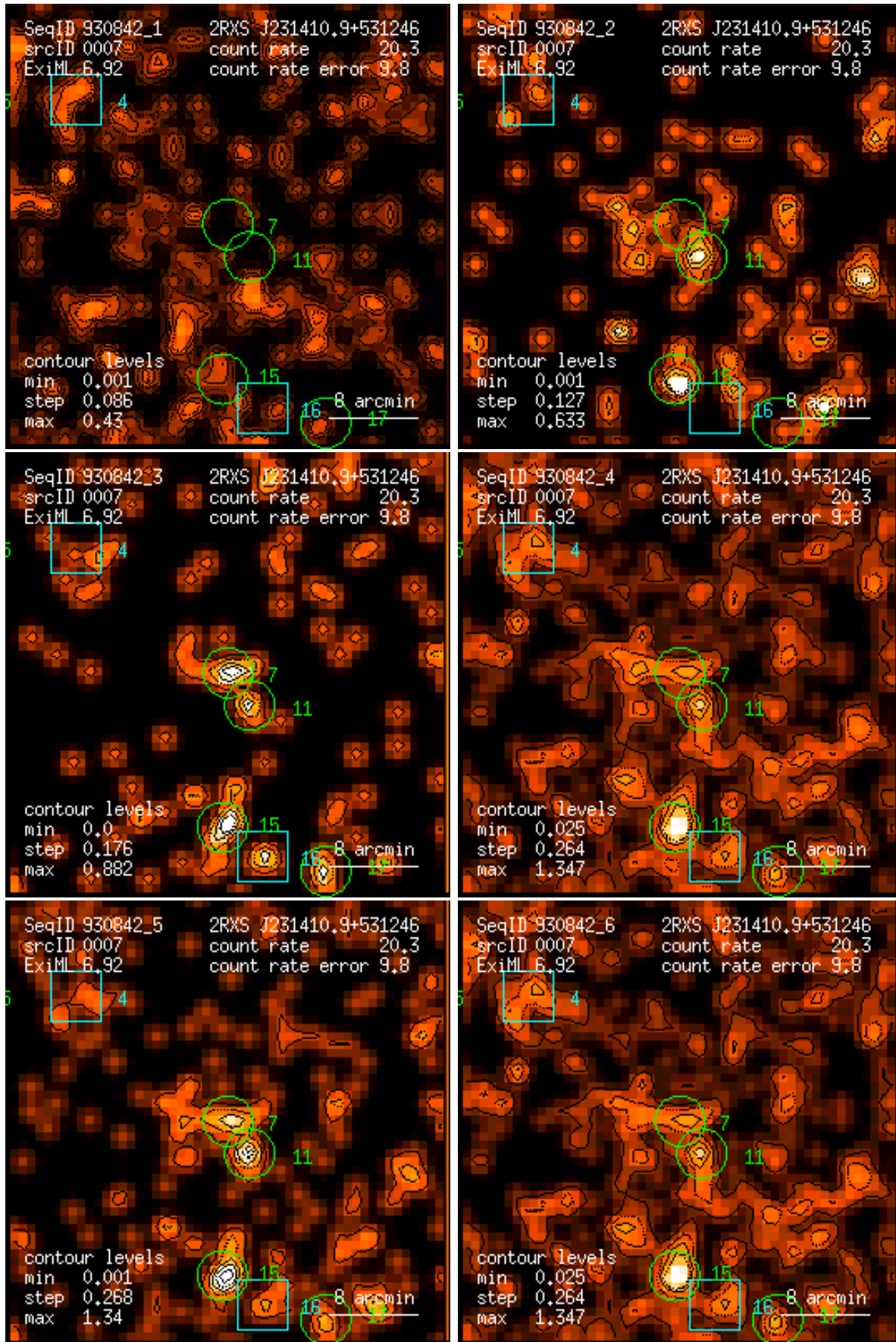
Figure 7: RASS 930842: detection 0007: band rate images, Gaussian filter: (1) PSPC channels 11 – 41, (2) 52 – 90, (3) 91 – 201, (4) 11 – 235, (5) 52 – 201, (6) 11 – 201. Broad band rates in counts/ks. Band rate contour levels in counts/ks/arcmin 2 .
