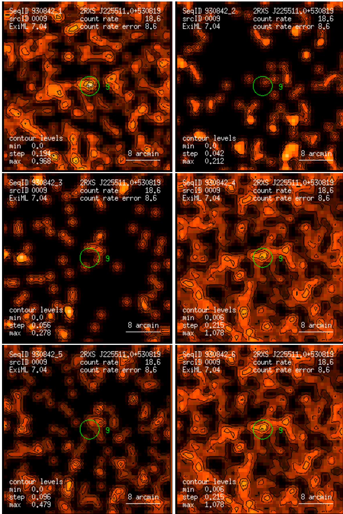
Figure 9: RASS 930842: detection 0009: band rate images, Gaussian filter: (1) PSPC channels 11 – 41, (2) 52 – 90, (3) 91 – 201, (4) 11 – 235, (5) 52 – 201, (6) 11 – 201. Broad band rates in counts/ks. Band rate contour levels in counts/ks/arcmin 2 .
