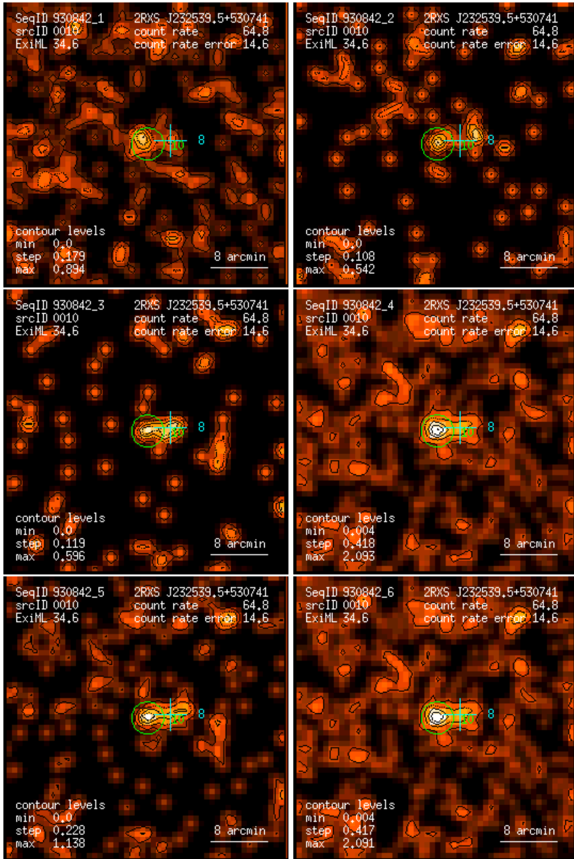
Figure 10: RASS 930842: detection 0010: band rate images, Gaussian filter: (1) PSPC channels 11 – 41, (2) 52 – 90, (3) 91 – 201, (4) 11 – 235, (5) 52 – 201, (6) 11 – 201. Broad band rates in counts/ks. Band rate contour levels in counts/ks/arcmin 2 .
