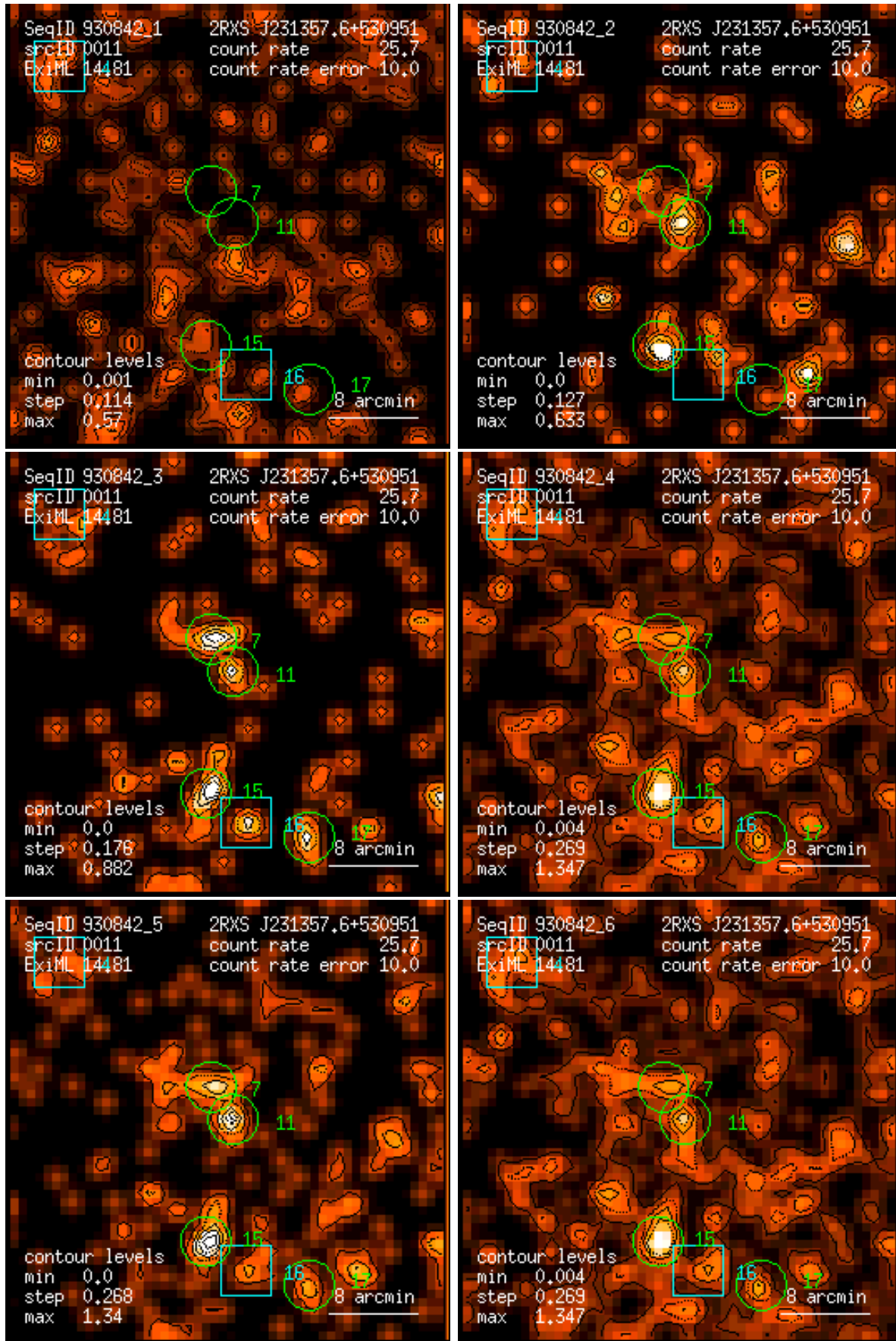
Figure 11: RASS 930842: detection 0011: band rate images, Gaussian filter: (1) PSPC channels 11 – 41, (2) 52 – 90, (3) 91 – 201, (4) 11 – 235, (5) 52 – 201, (6) 11 – 201. Broad band rates in counts/ks. Band rate contour levels in counts/ks/arcmin 2 .
