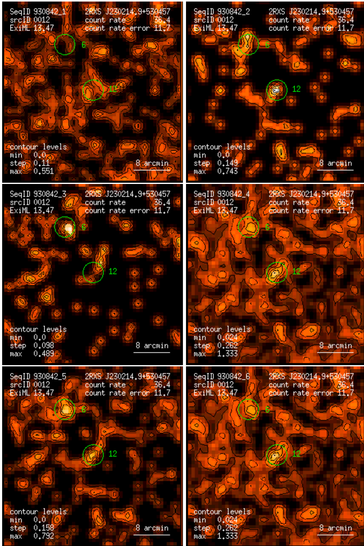
Figure 12: RASS 930842: detection 0012: band rate images, Gaussian filter: (1) PSPC channels 11 – 41, (2) 52 – 90, (3) 91 – 201, (4) 11 – 235, (5) 52 – 201, (6) 11 – 201. Broad band rates in counts/ks. Band rate contour levels in counts/ks/arcmin 2 .
