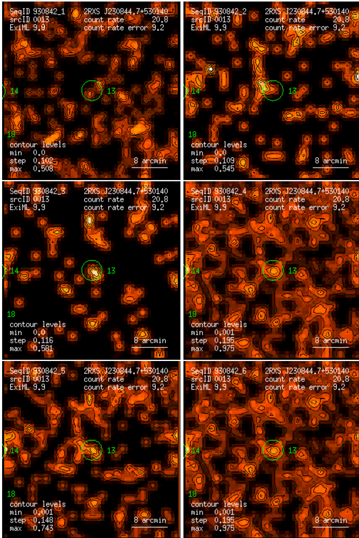
Figure 13: RASS 930842: detection 0013: band rate images, Gaussian filter: (1) PSPC channels 11 – 41, (2) 52 – 90, (3) 91 – 201, (4) 11 – 235, (5) 52 – 201, (6) 11 – 201. Broad band rates in counts/ks. Band rate contour levels in counts/ks/arcmin 2 .
