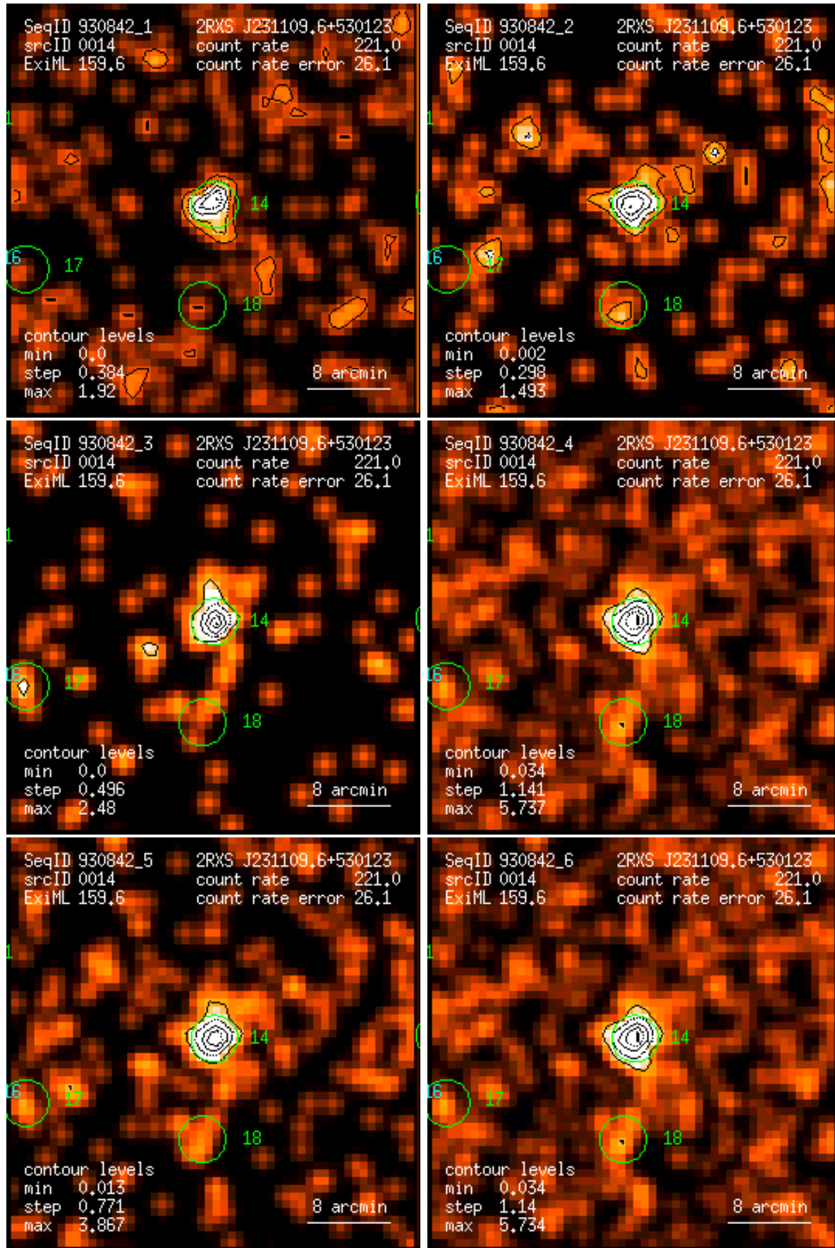
Figure 14: RASS 930842: detection 0014: band rate images, Gaussian filter: (1) PSPC channels 11 – 41, (2) 52 – 90, (3) 91 – 201, (4) 11 – 235, (5) 52 – 201, (6) 11 – 201. Broad band rates in counts/ks. Band rate contour levels in counts/ks/arcmin 2 .
