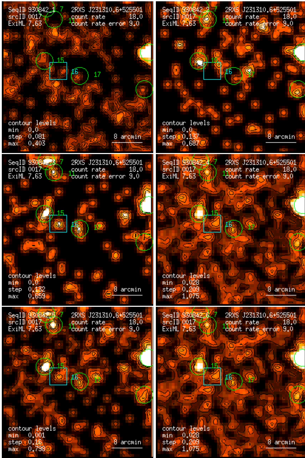
Figure 17: RASS 930842: detection 0017: band rate images, Gaussian filter: (1) PSPC channels 11 – 41, (2) 52 – 90, (3) 91 – 201, (4) 11 – 235, (5) 52 – 201, (6) 11 – 201. Broad band rates in counts/ks. Band rate contour levels in counts/ks/arcmin 2 .
