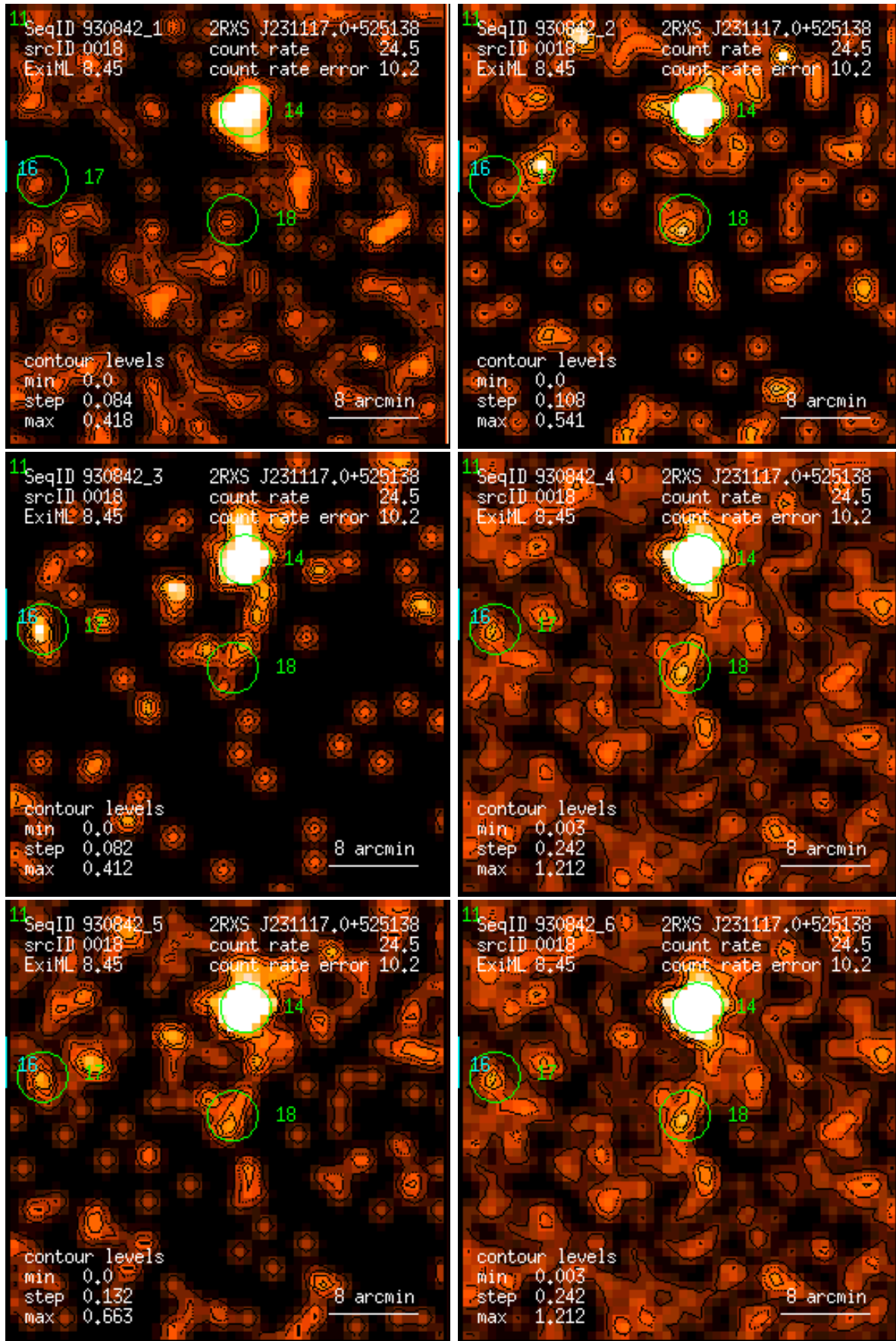
Figure 18: RASS 930842: detection 0018: band rate images, Gaussian filter: (1) PSPC channels 11 – 41, (2) 52 – 90, (3) 91 – 201, (4) 11 – 235, (5) 52 – 201, (6) 11 – 201. Broad band rates in counts/ks. Band rate contour levels in counts/ks/arcmin 2 .
