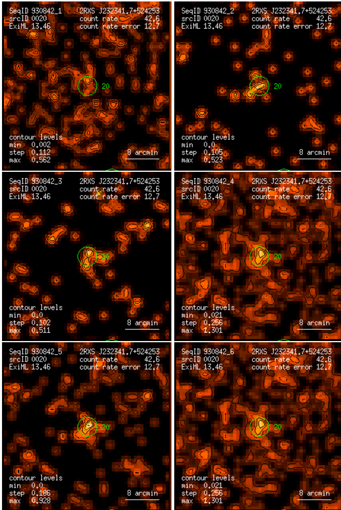
Figure 20: RASS 930842: detection 0020: band rate images, Gaussian filter: (1) PSPC channels 11 – 41, (2) 52 – 90, (3) 91 – 201, (4) 11 – 235, (5) 52 – 201, (6) 11 – 201. Broad band rates in counts/ks. Band rate contour levels in counts/ks/arcmin 2 .
